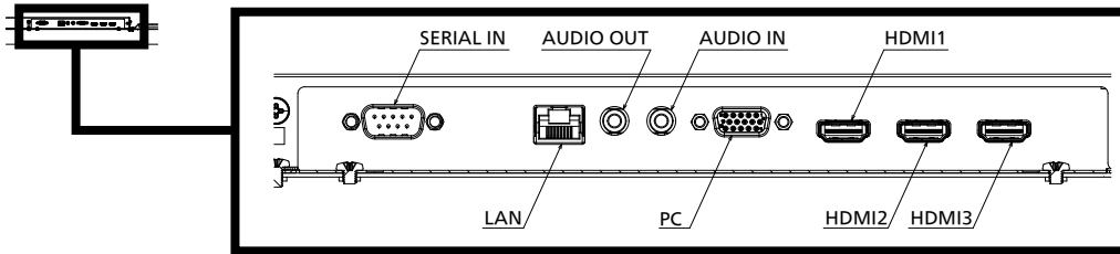
Sectional view of terminal a (SERIAL IN / LAN / AUDIO OUT / AUDIO IN / PC / HDMI 1/2/3)
