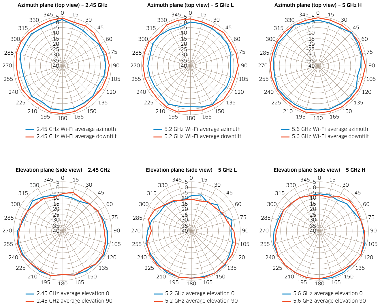
Figures. OmniAccess AP1351 antenna pattern plots
