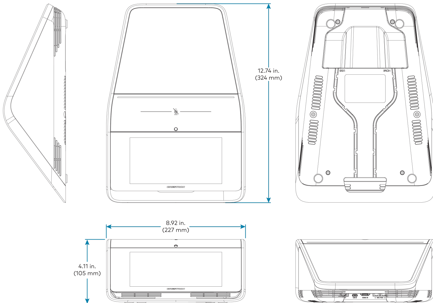
Crestron Flex Tabletop Conference Device (CCS-UC-1-X-T-V)
