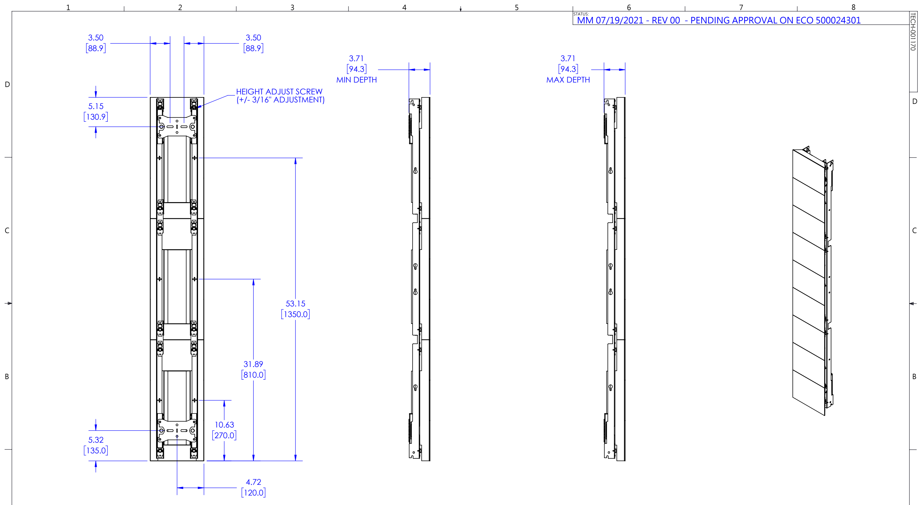
TILD1X3IERF MOUNT WITH SAMSUNG IER-F DISPLAYS (REAR VIEW)
