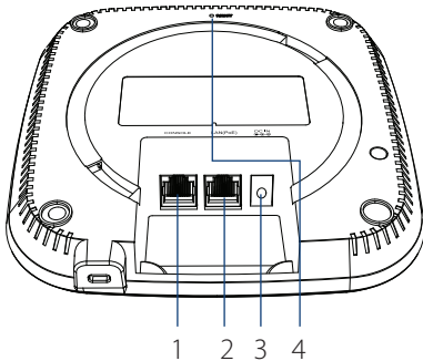
Figure 2: Rear Connectors
