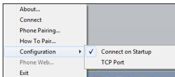
Figure 7-16: TCP Port
