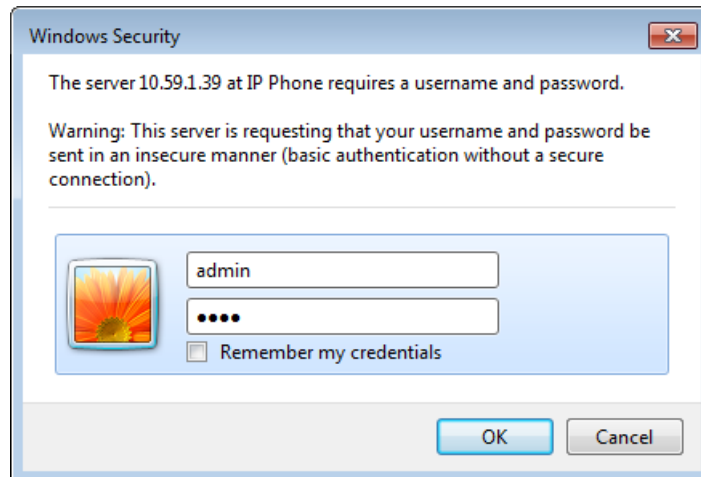
Figure 3-8: Login
