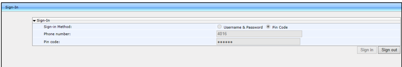
Figure 3-13: Sign-out
