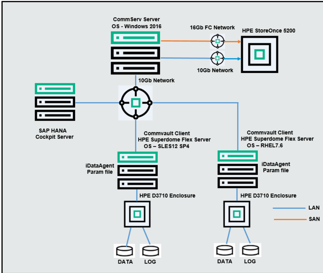
FIGURE 1. SAP HANA scale-up backup environment using Commvault (tested lab configuration)
