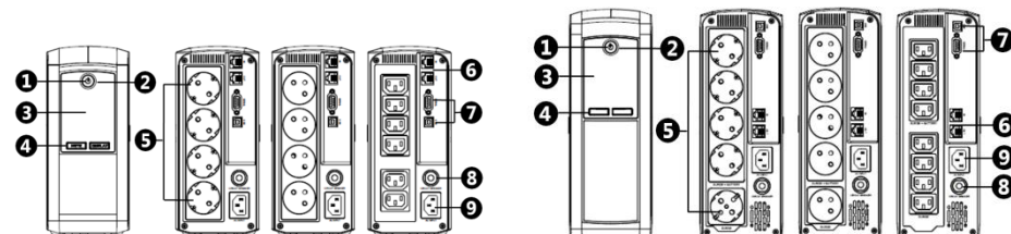
VP700/VP700EILCD/VP1000EILCD/VP1000EILCD (Schuko/French/IEC Outlet) VP1200/VP1200EILCD/VP1600EILCD/VP1600EILCD (Schuko/French/IEC Outlet)
