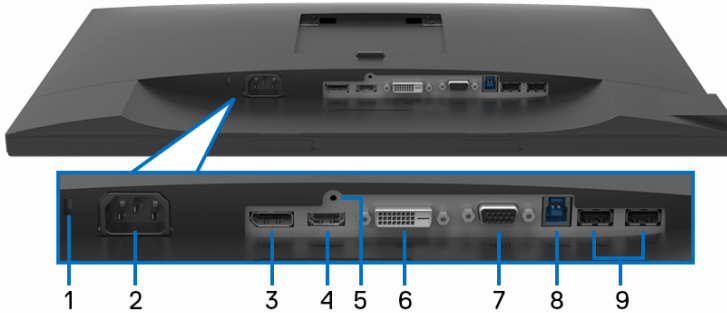
Bottom view without monitor stand
