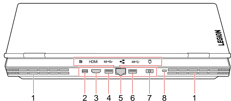
Figure 5. Lenovo Legion Y740–15/17 Series – rear view
