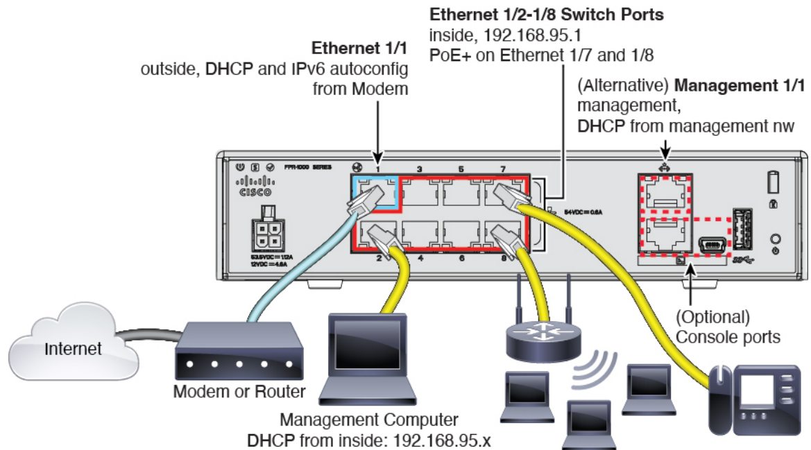
Figure 26: Cabling the Firepower 1010
