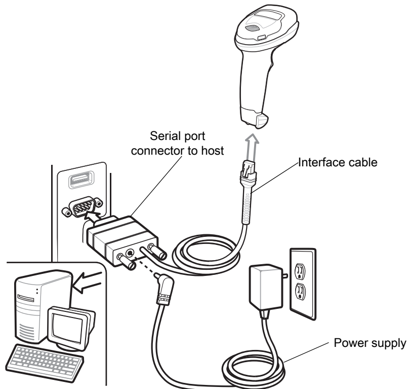
Figure 14 RS-232 Connection
