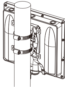
Figure 6: Mounting the Device
