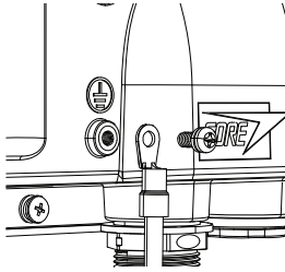
Figure 11: Attaching the Grounding Wire
