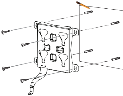
Figure 7: Attaching the Mounting Plate
