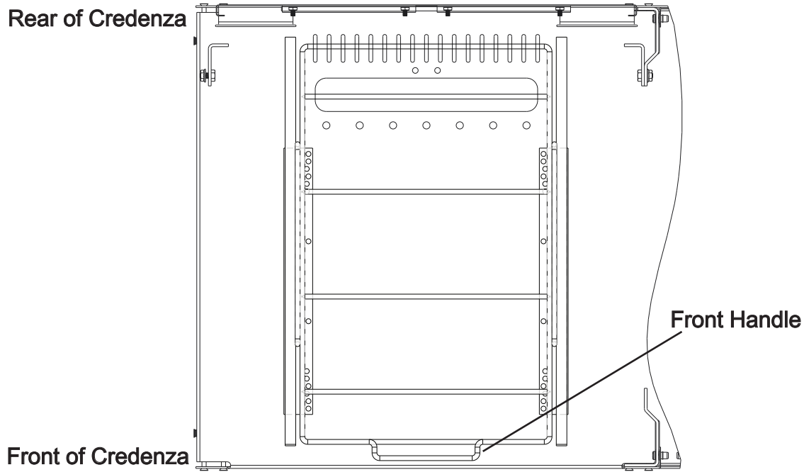
(FIGURE A) Top View of Frame and Runners Installed
