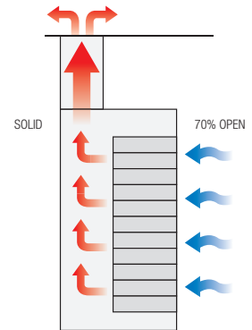
digital with passive chimney ventilation
