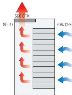
hybrid with top active ventilation
