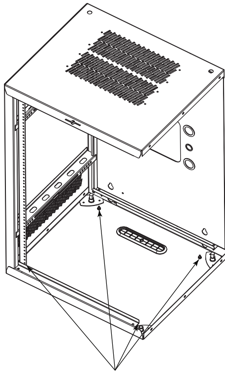
Bonding Studs (4) 10-32
