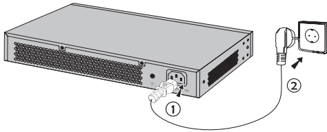
Figure 3-3 Connecting to Power Supply
