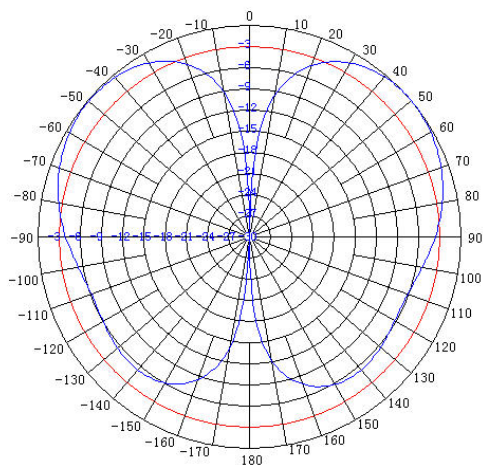
Vertical Radiation Pattern @ 2.4 GHz
