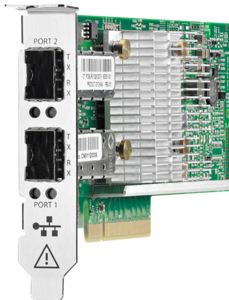
HPE Ethernet 10Gb 2-port 530SFP+ Adapter, with half-height bracket
