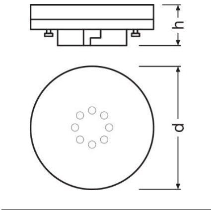
ST GX53 40 100° 4.7 W/827 GX53, ST GX53 40 100° 4.7 W/840 GX53
