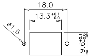
SUGGESTED PANEL CUTOUT
