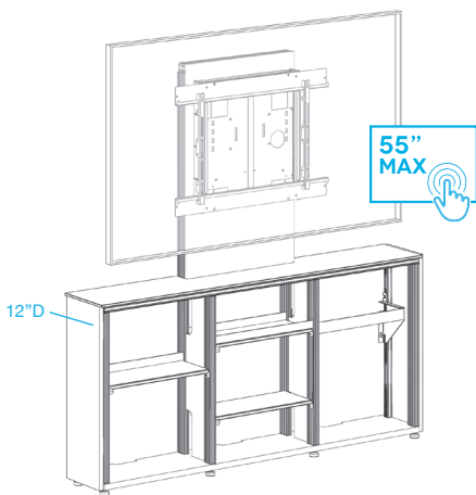
3-Bay, Low-Profile Wall Cabinet EZ-Touch Lift Mount D1/337AL/
