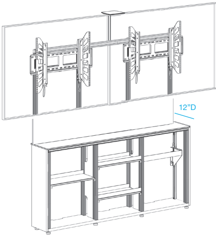
3-Bay, Low-Profile Wall Cabinet Dual Monitor Bundle D1/337AM2/
