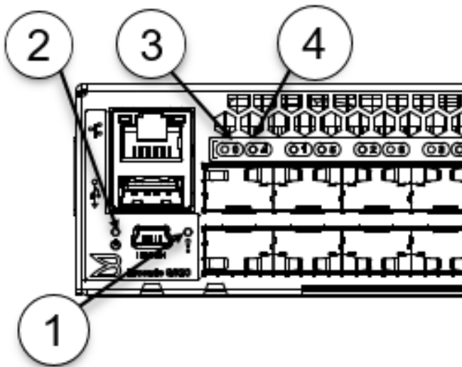
Figure 29: Brocade G620 Port-Side LEDs
