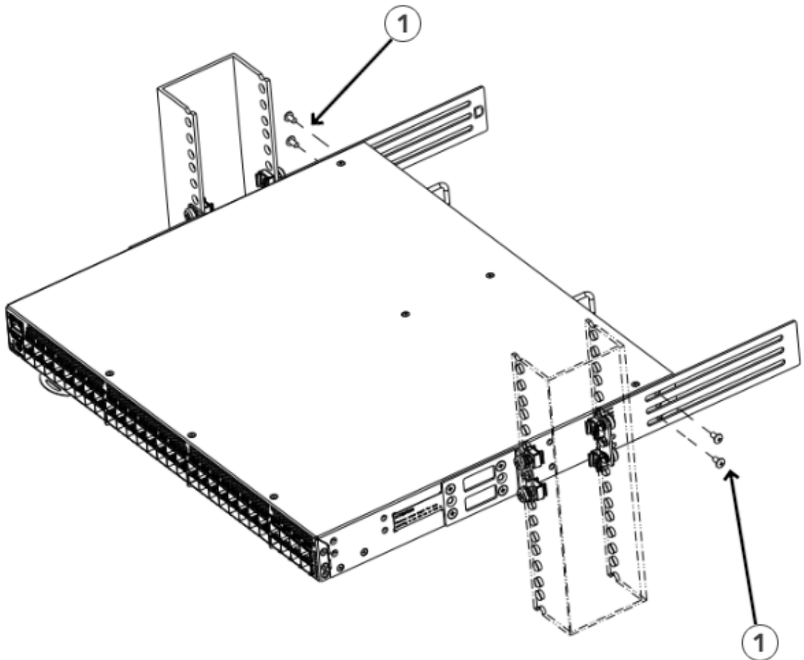
Figure 24: Attaching the Rear Brackets to the Device
