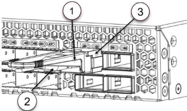
Figure 27: Installing a QSFP Transceiver in an Upper Port
