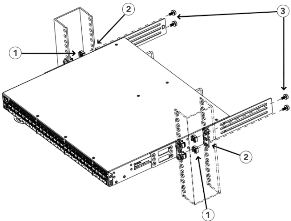
Figure 23: Attaching the Rear Brackets to the Rack
