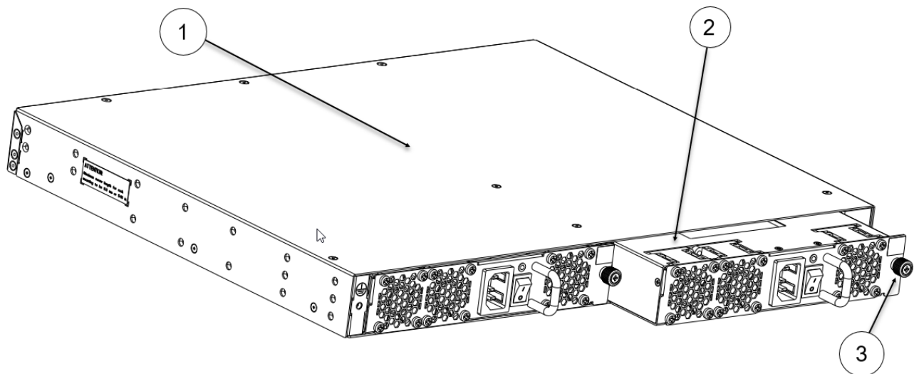
Figure 32: Inserting an AC Power Supply and Fan Assembly
