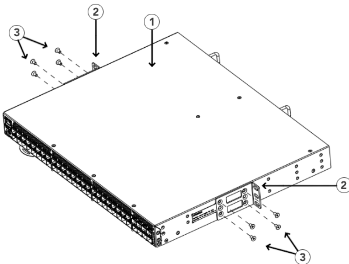
Figure 21: Attaching the Front Brackets
