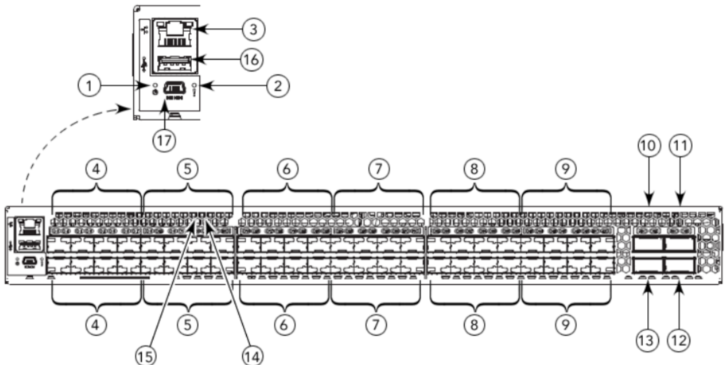
Figure 2: Port-Side View of G620 Version 2
