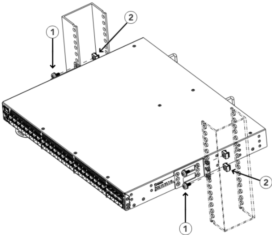
Figure 22: Attaching the Front Brackets to the Rack
