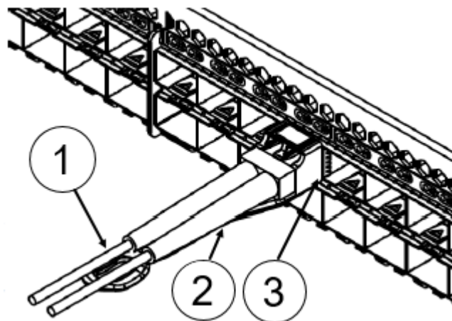
Figure 25: Closeup of Installing a 32Gb/s SFP+ Transceiver into an Upper Port
