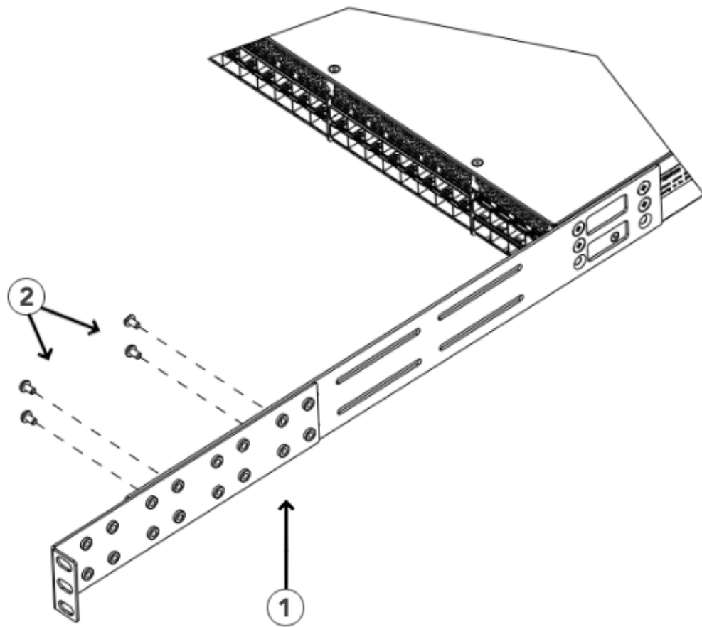
Figure 14: Attaching the Short or Long Rear Brackets to the Extensions
