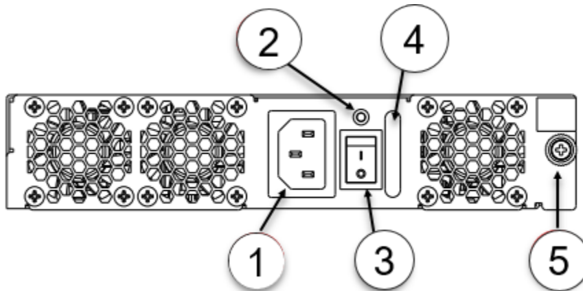
Figure 30: AC Power Supply and Fan Assembly
