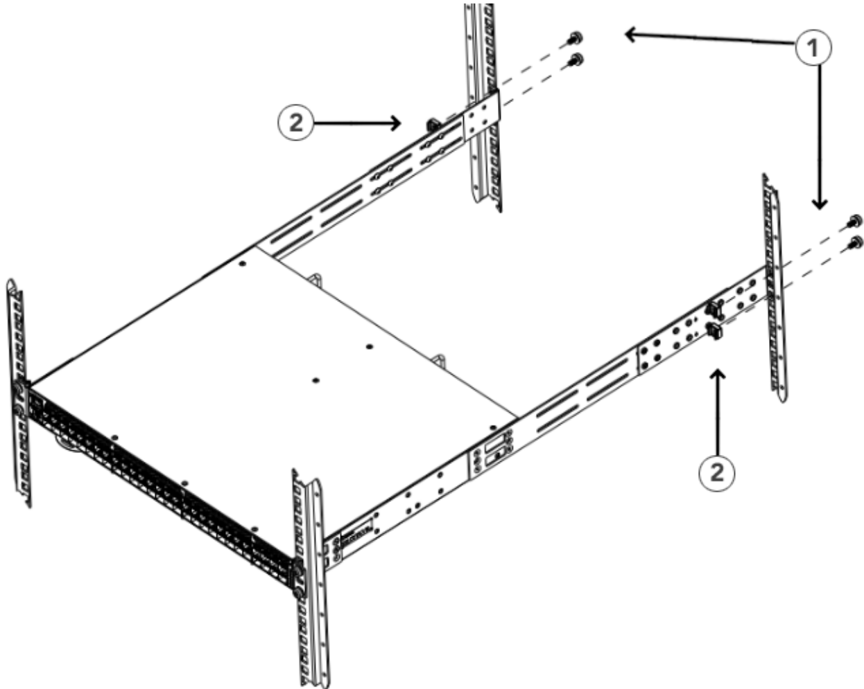
Figure 9: Attaching the Rear Brackets to the Rack Posts
