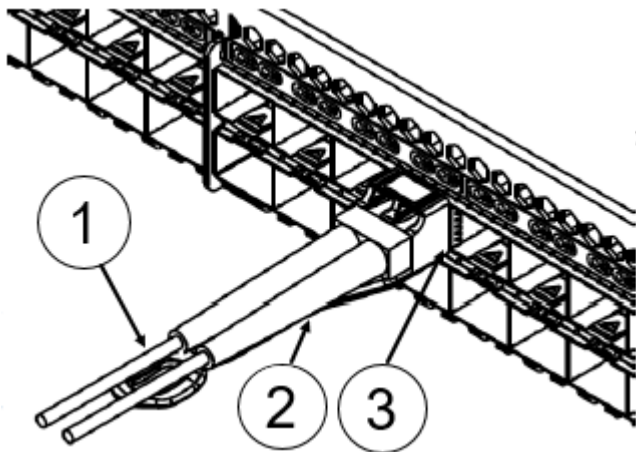
Figure 26: Replacing an SFP+ Optical Transceiver in an Upper Port
