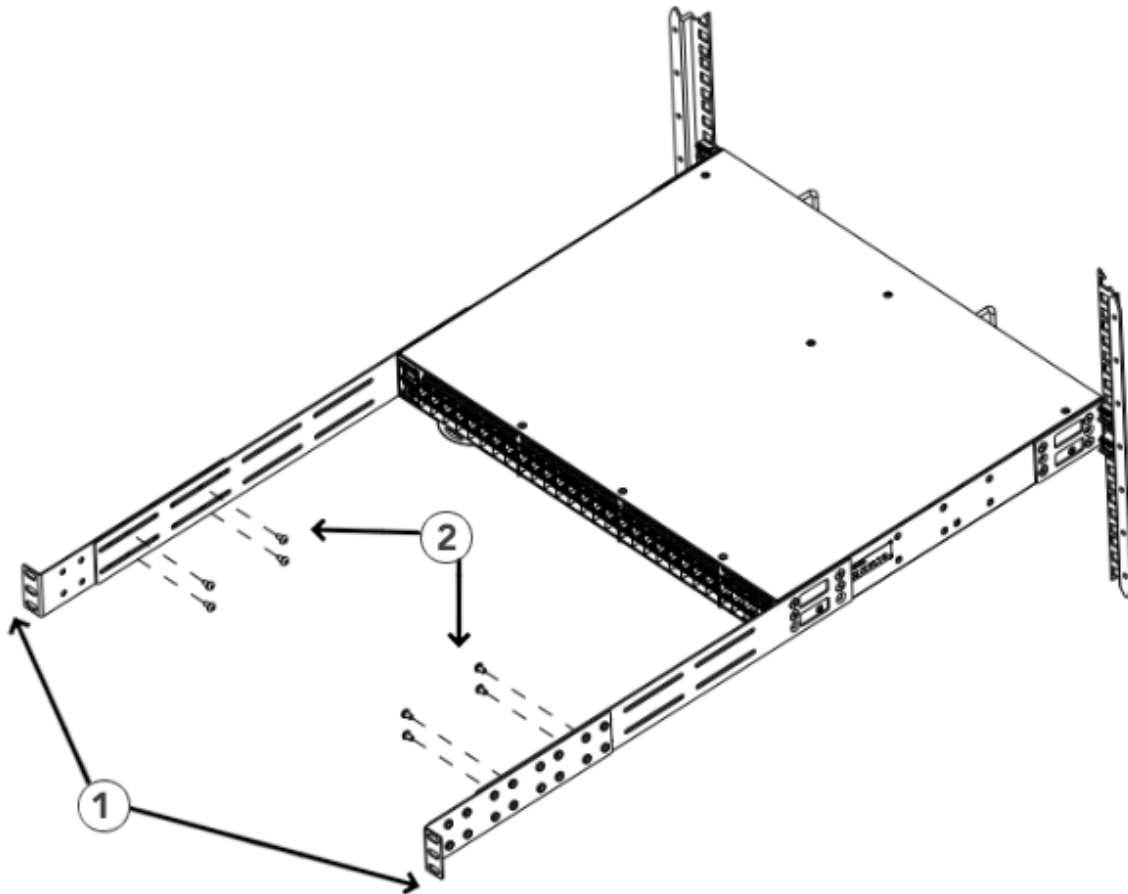
Figure 13: Attaching the Rear Brackets to the Extensions at the Front of the Device
