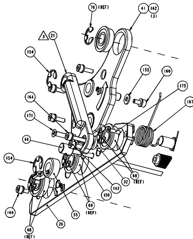
DETAIL A
