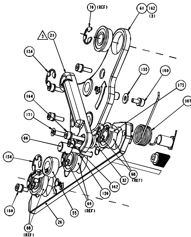
DETAIL A
