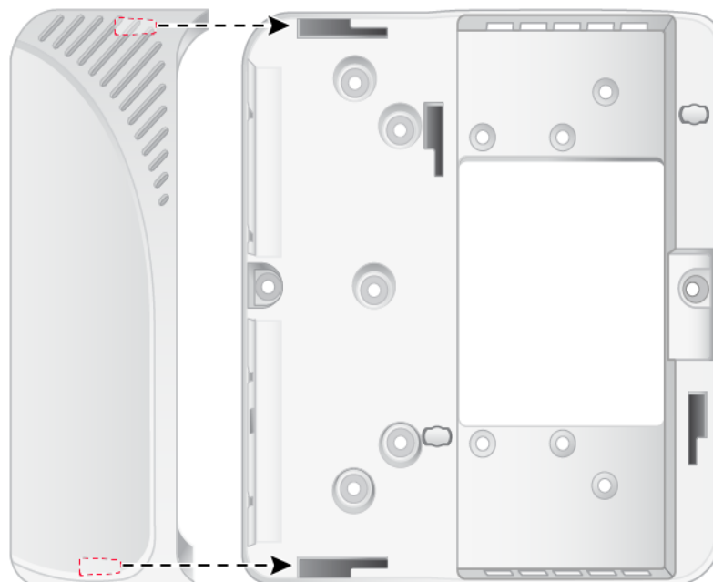
Figure 5 Fitting Front Cover onto Wall Mount
