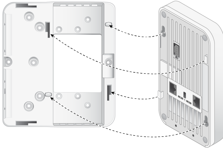
Figure 4 Securing AP-205H to Wall Mount
