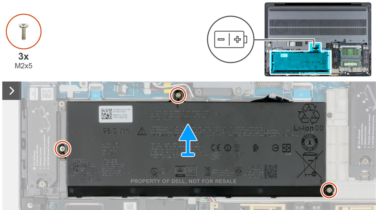
Figure 44. Removing the battery
