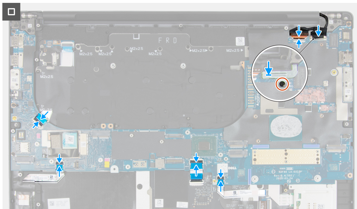
Figure 112. Installing the system board
