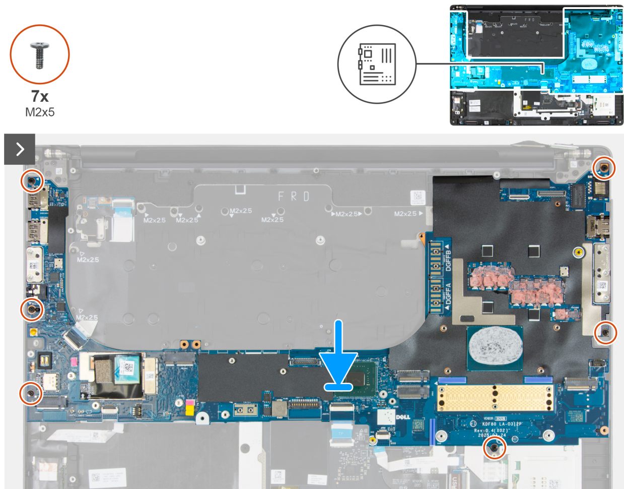
Figure 111. Installing the system board
