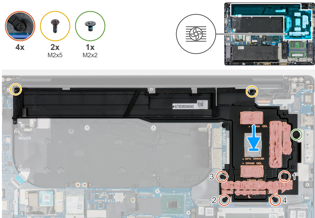
Figure 76. Installing the heat sink for computers shipped with discrete graphics
