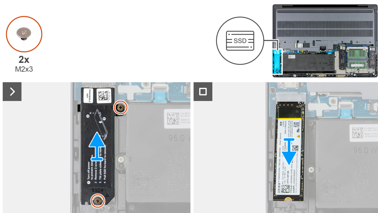
Figure 40. Removing the M.2 2280 SSD from slot 4 (SSD4)
