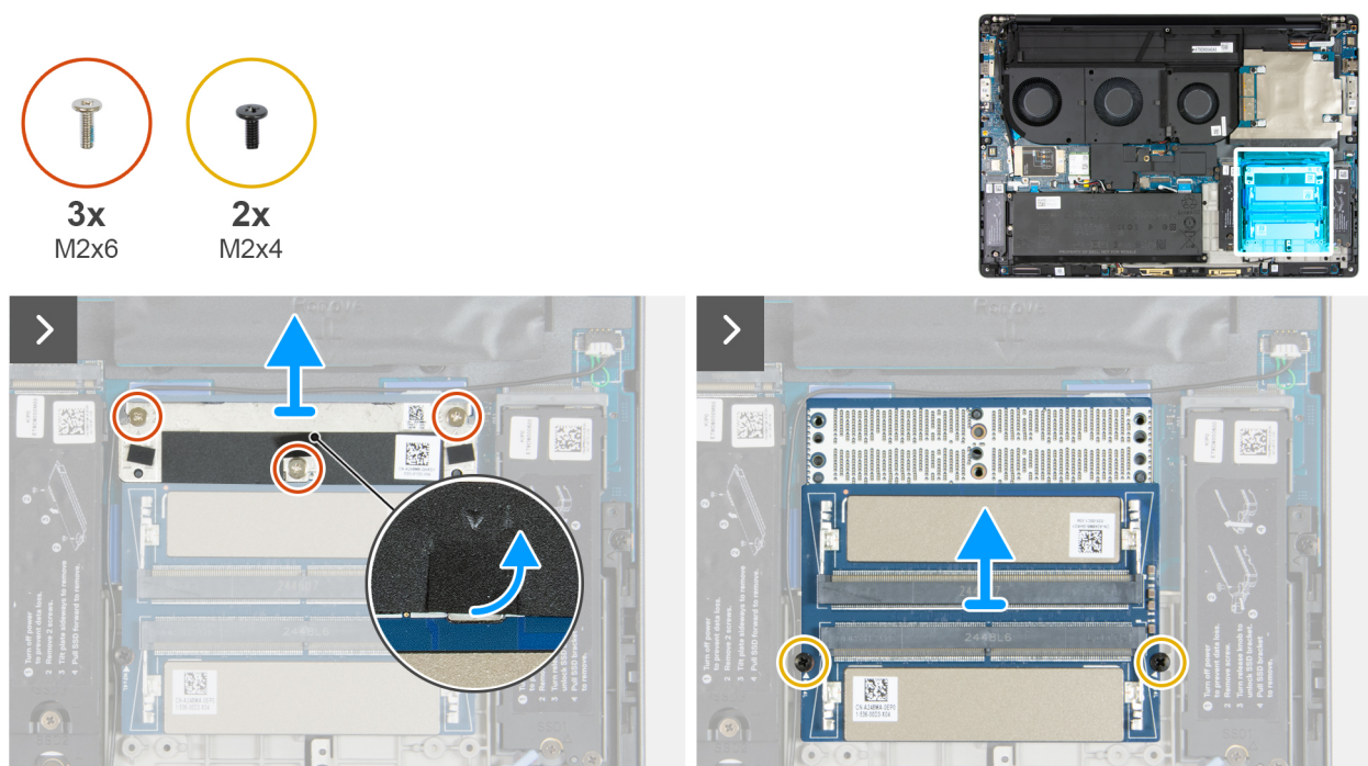
Figure 67. Removing the memory interposer board
