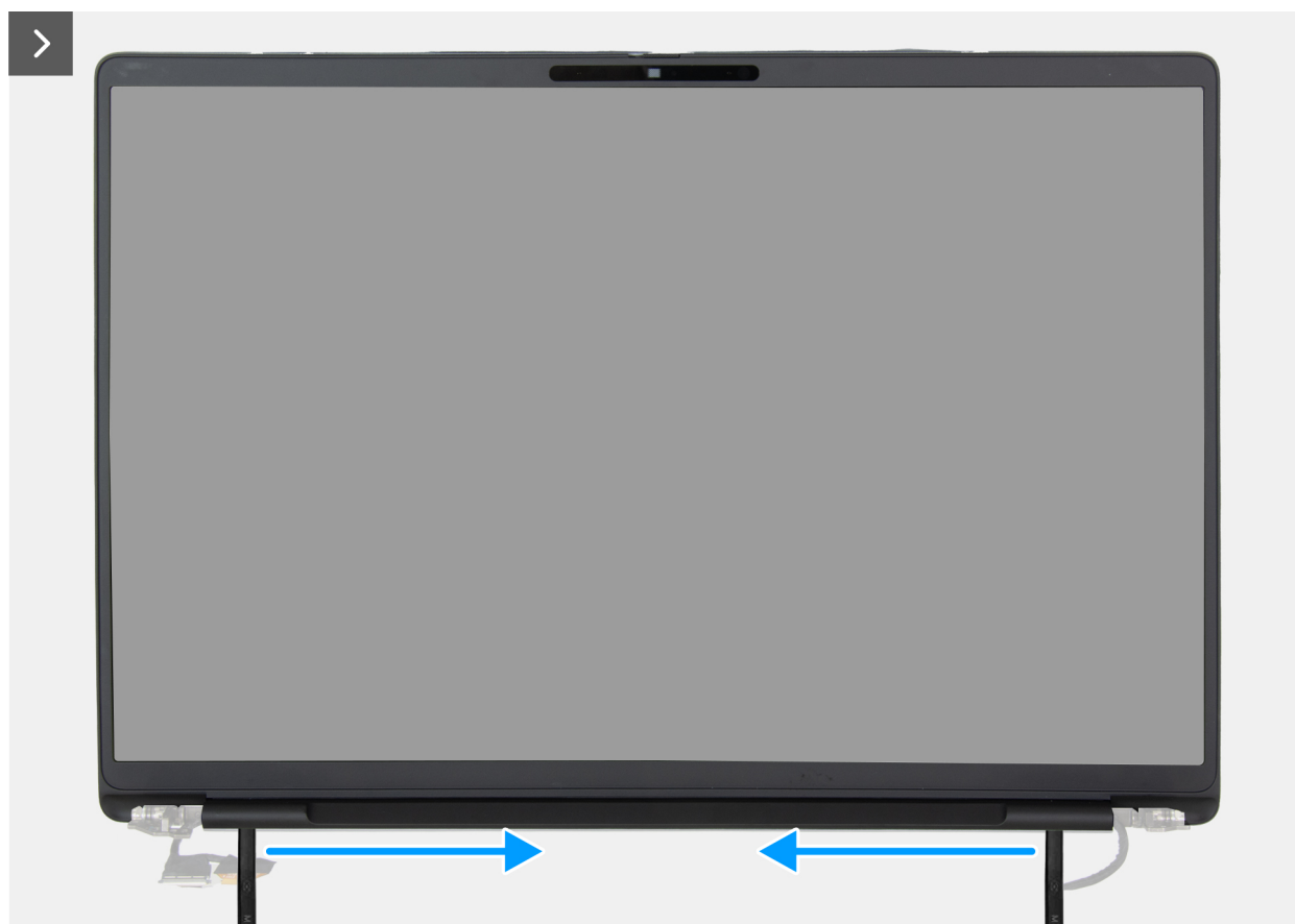
Figure 86. Removing the display bezel
