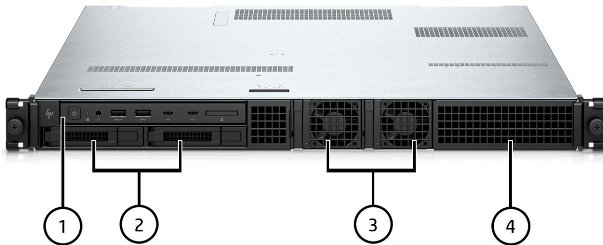
Front view
