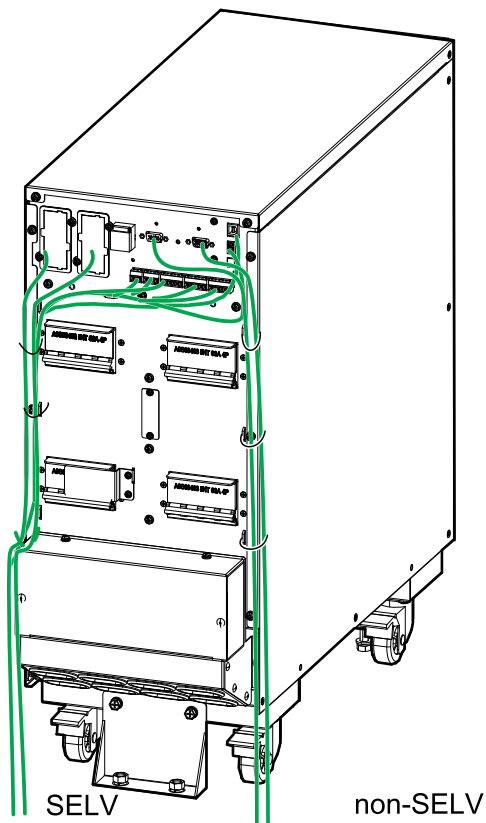
SELV and Non-SELV Cable Routing for 10 - 20 kVA 3:1 UPS
