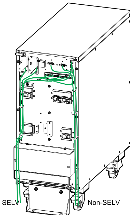
SELV and Non-SELV Cable Routing for 10 - 20 kVA 3:1 UPS
