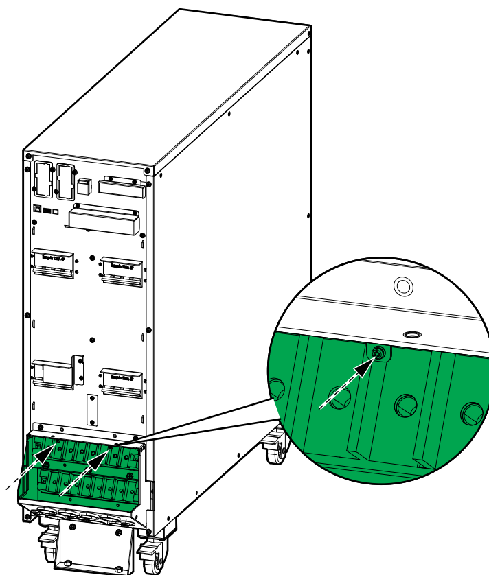
Rear View of 30-40 kVA 3:3 UPS
