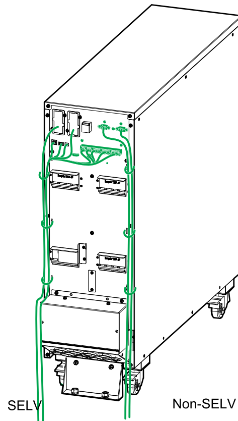
SELV and Non-SELV Cable Routing for 30 - 40 kVA 3:3 UPS
