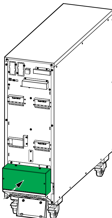
Rear View of 30-40 kVA 3:3 UPS
