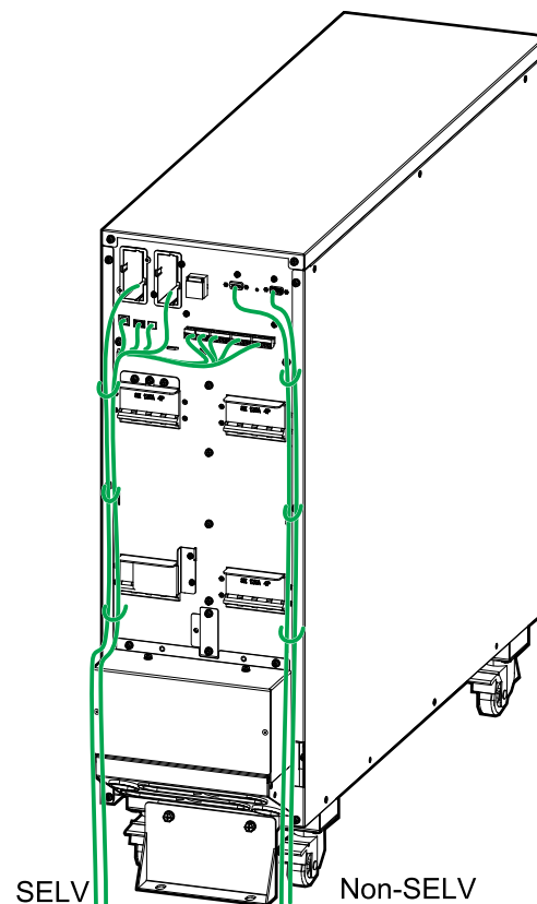
SELV and Non-SELV Cable Routing for 30 kVA 3:1 UPS
