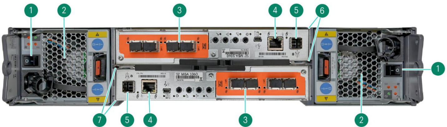
HPE MSA 1060 Storage-Rear View
