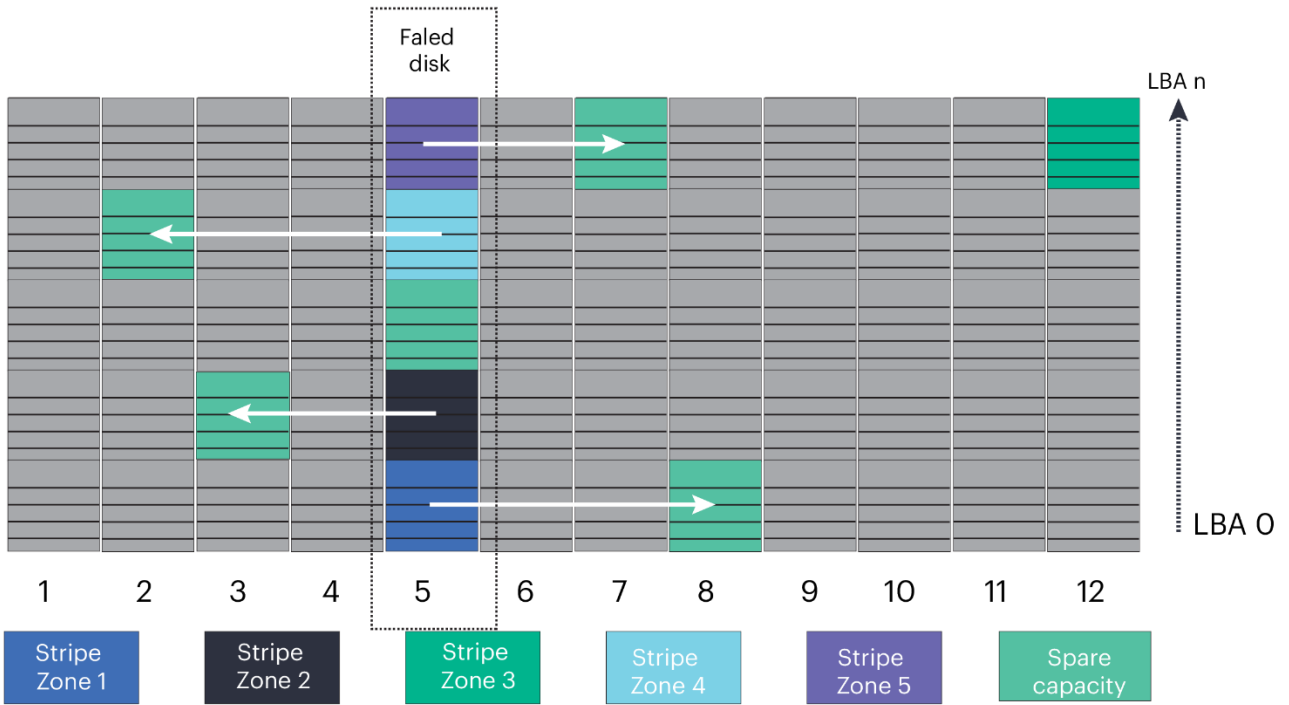
Figure 23. Example of rebuilding data located on a failed drive to spare capacity
