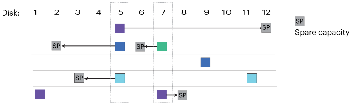
Figure 25. MSA-DP+ double disk failure rebuild Stage 2 is to return the disk group to a fault-tolerant state
