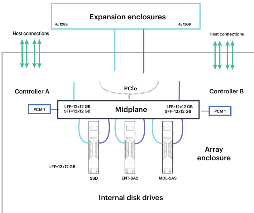
Figure 4. HPE MSA array architecture
