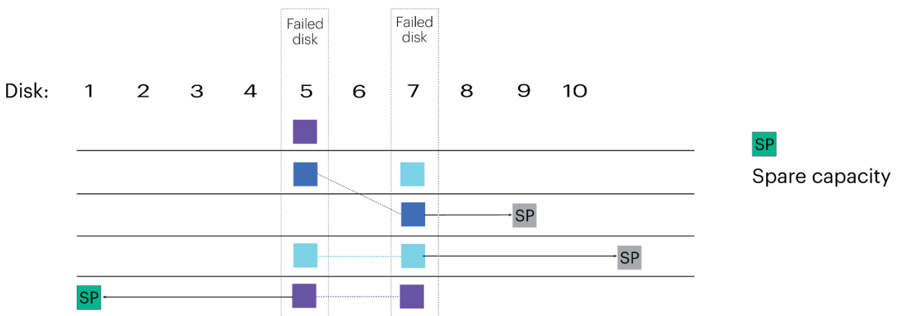
Figure 24. MSA-DP+ double disk failure rebuild Stage 1 is to protect critical stripe zones
