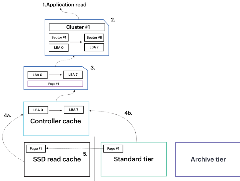
Figure 15. Read mechanism
