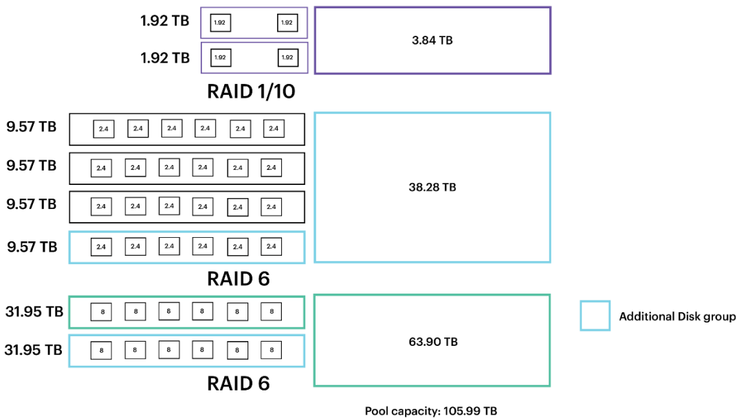
Figure 31. Example of pool layout after capacity expansion by adding additional disk groups
