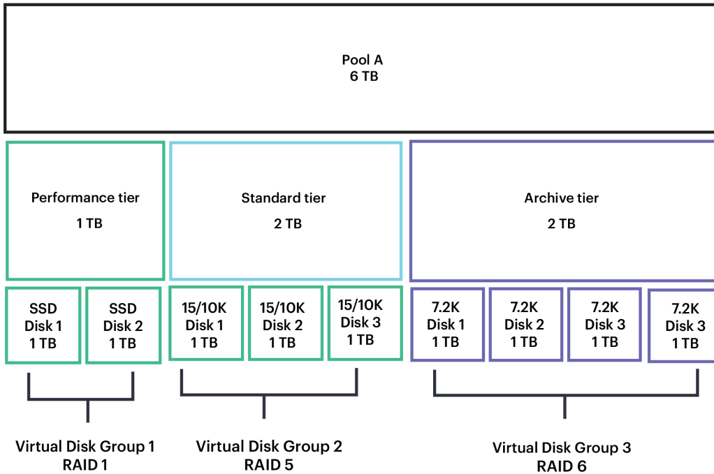
Figure 16. Representation of a multitiered pool layout
