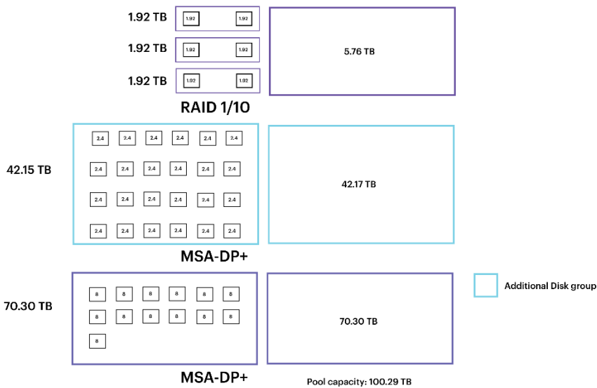
Figure 33. Example of pool layout using MSA-DP+ HDD disk groups after capacity expansion
