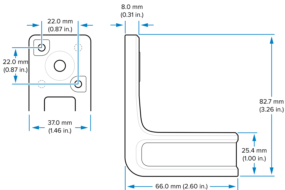
Figure 4 L-Bracket Dimensions
