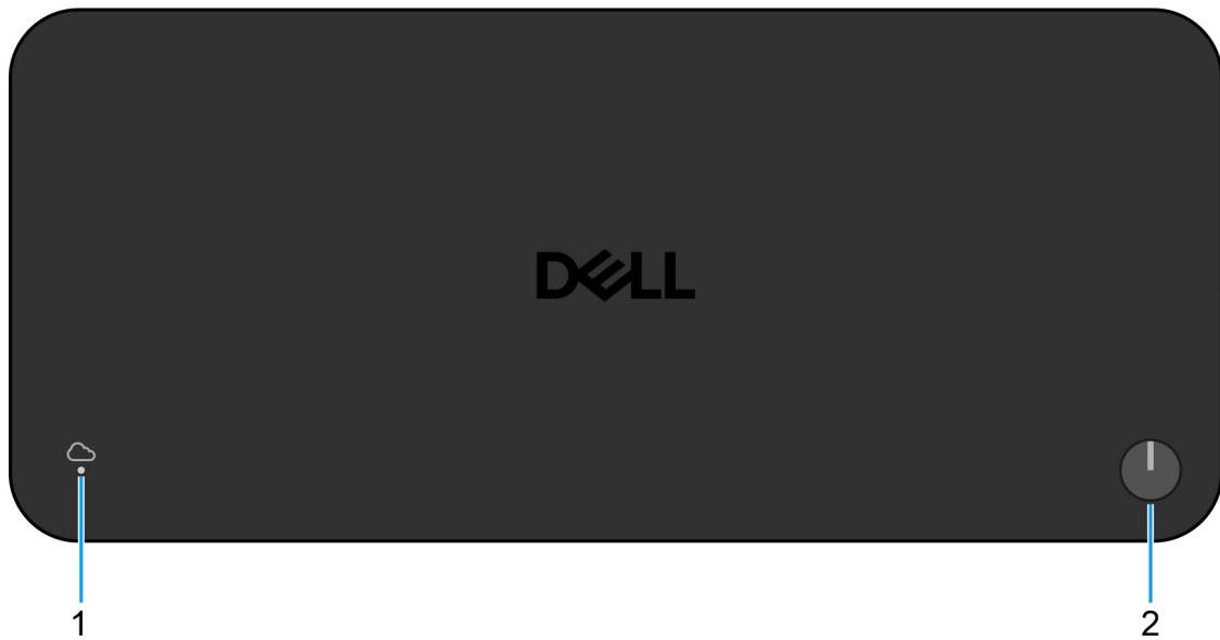
Figure 3. Dell Pro Thunderbolt 4 Smart dock SD25TB4 top view
