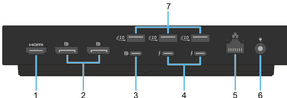
Figure 7. Back view
