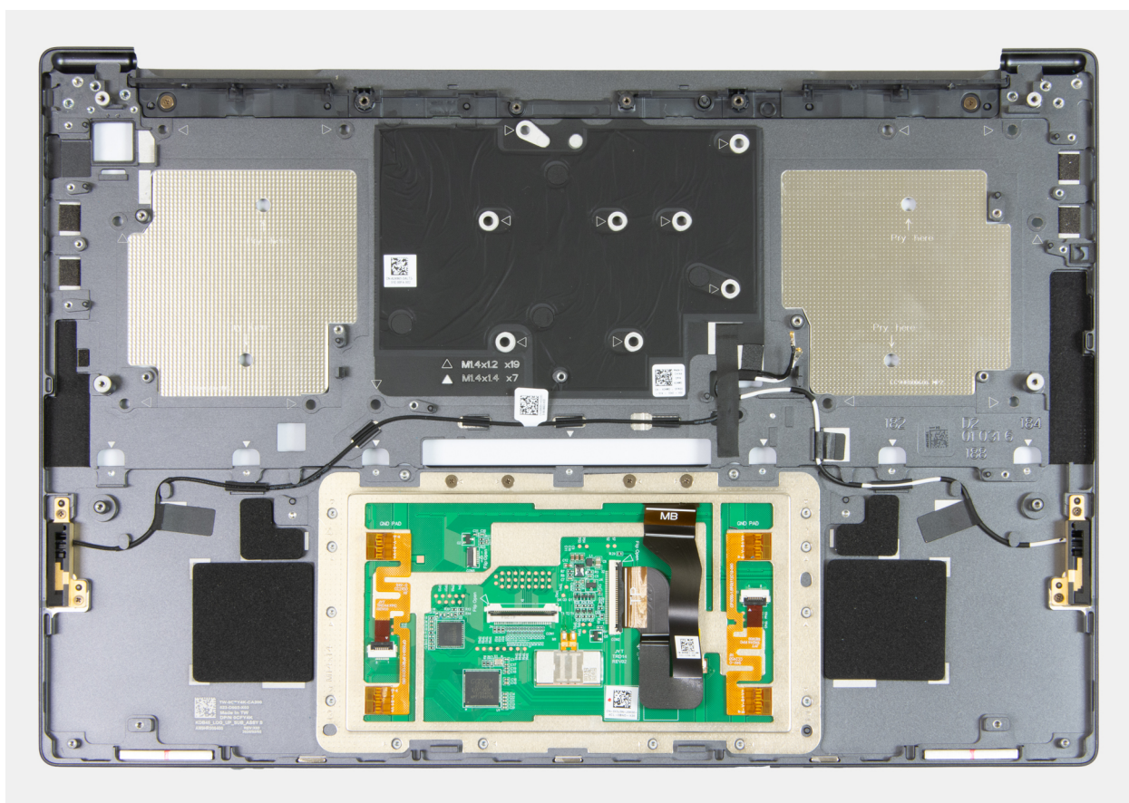
Figure 79. Palm rest and touchpad assembly
