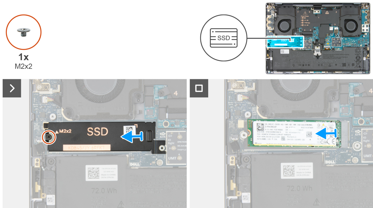
Figure 23. Removing the M.2 2280 solid state drive
