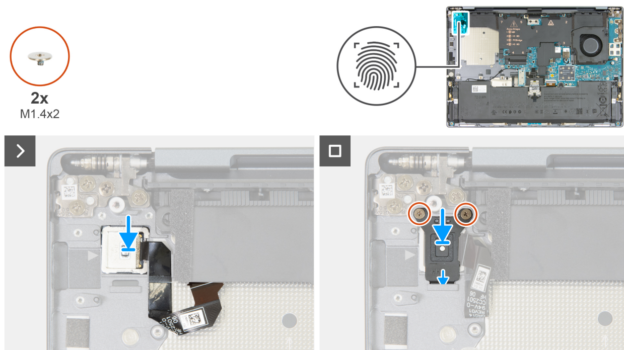
Figure 68. Installing the power button or fingerprint reader
