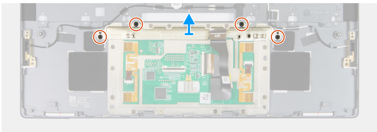
Figure 77. Removing the touchpad bracket
