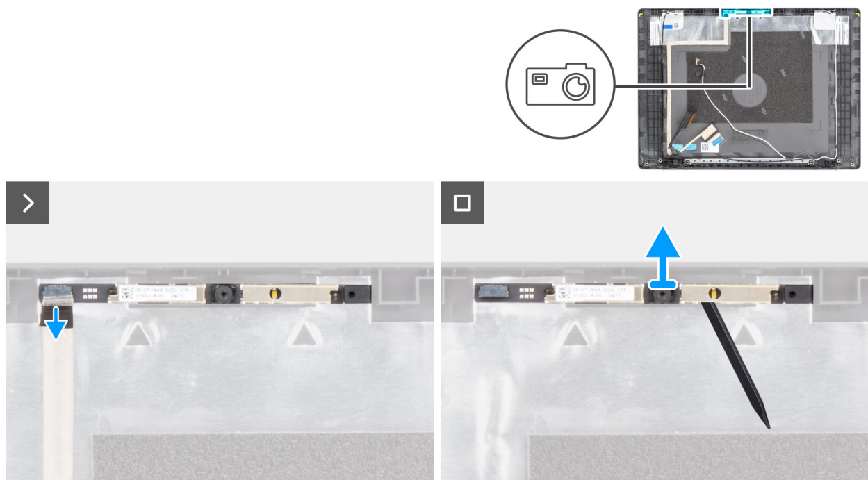
Figure 74. Removing the camera
