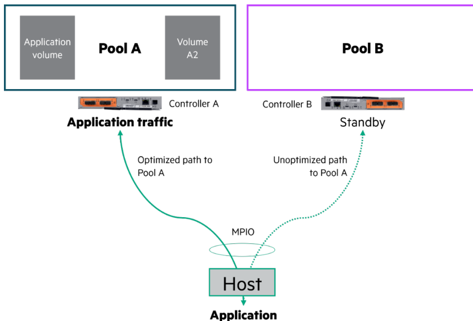
Figure 5. Example of a host with redundant paths to a volume
