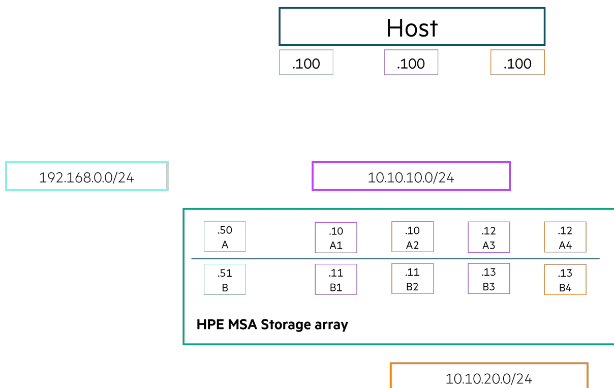
Figure 2. Example of iSCSI network subnet assignments
