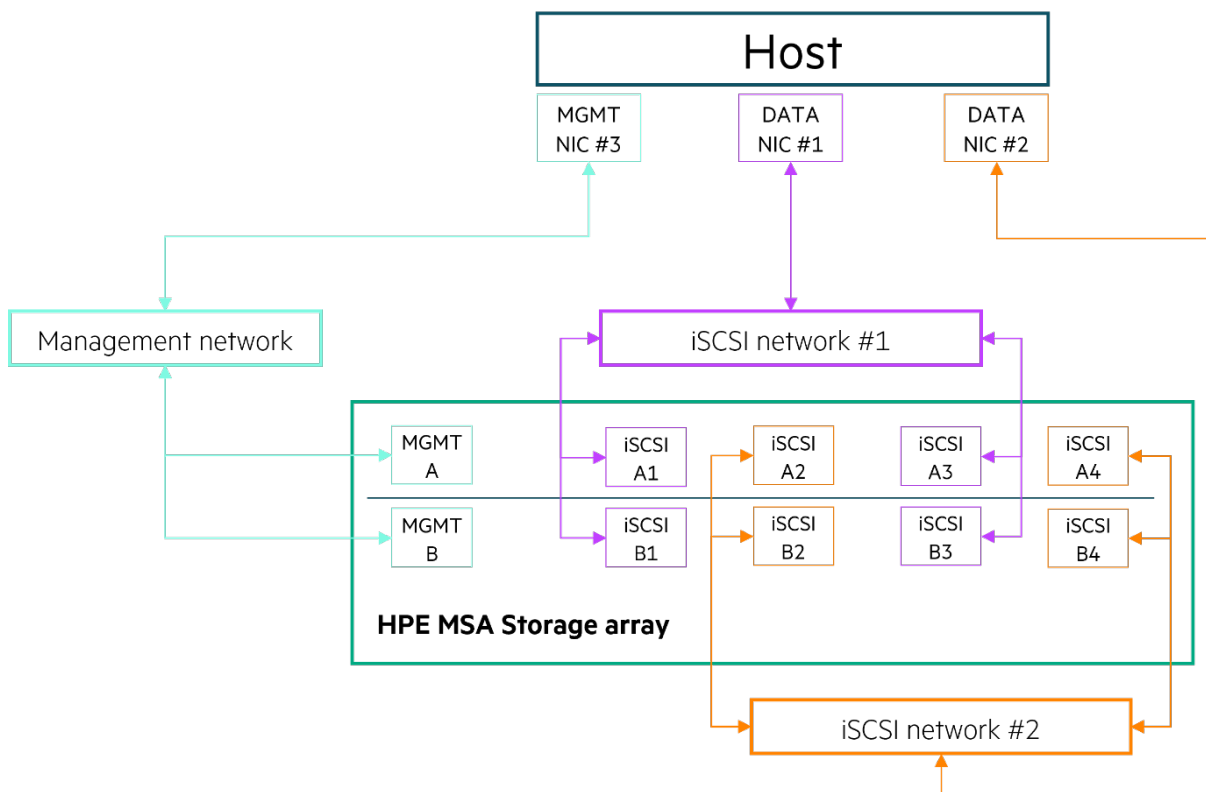
Figure 1. A sample iSCSI network topography
