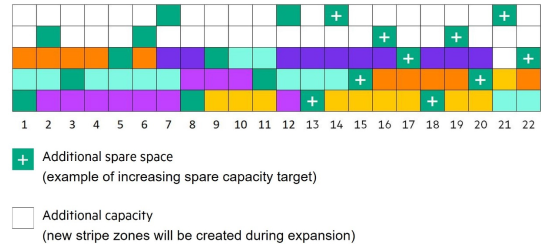
Figure 34 demonstrates the expansion of capacity in addition to the increase of spare capacity by adding ten more drives to the disk group.
