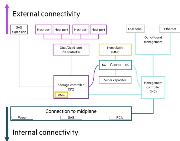
Figure 3. Simplified HPE MSA controller diagram
