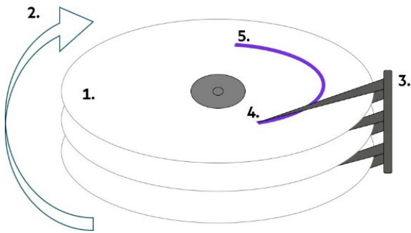
Figure 18. Internal view of a disk drive processing a sequential read/write operation
