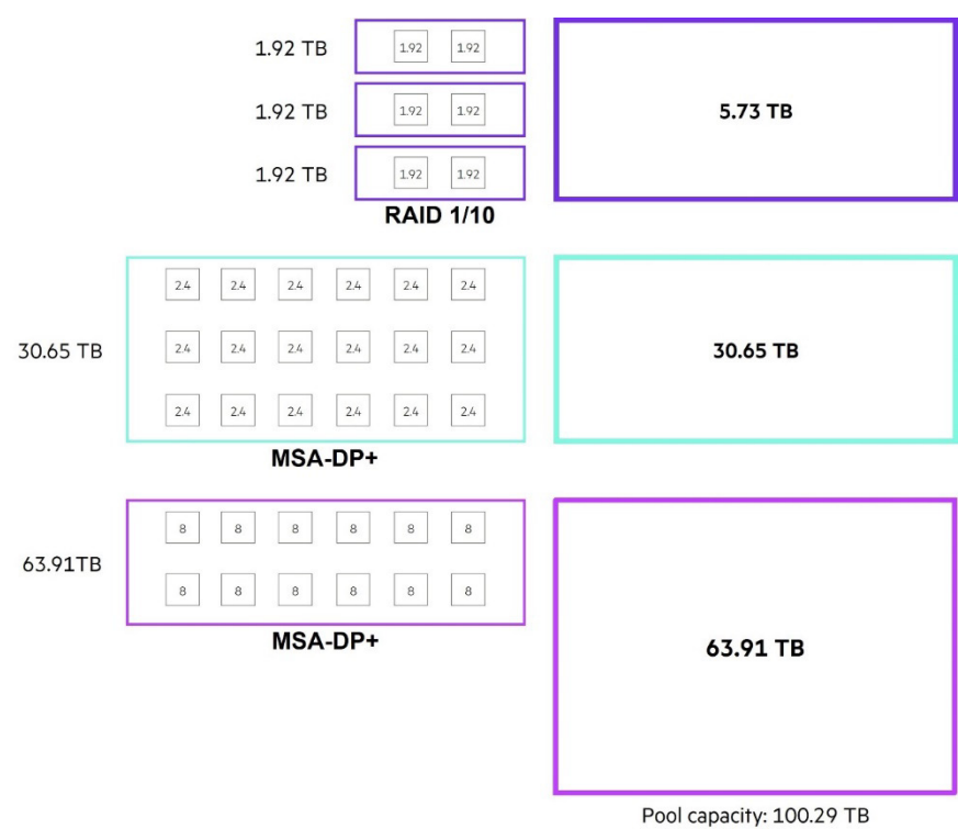
Figure 32. Example of pool layout using MSA-DP+ HDD disk groups before capacity expansion
