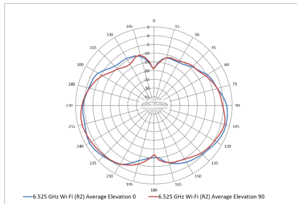
6.56 GHz Wi-Fi antennas patterns (vertical)
