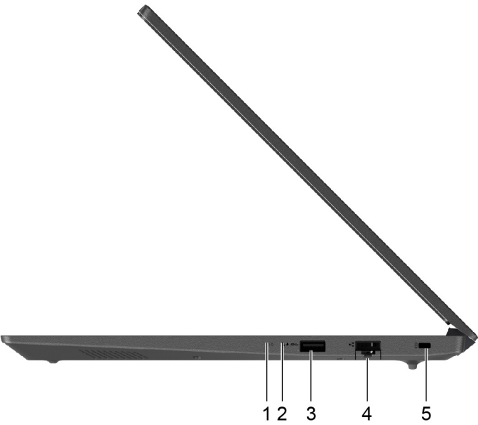
Figure 7. 15.6-inch models—right-side view
