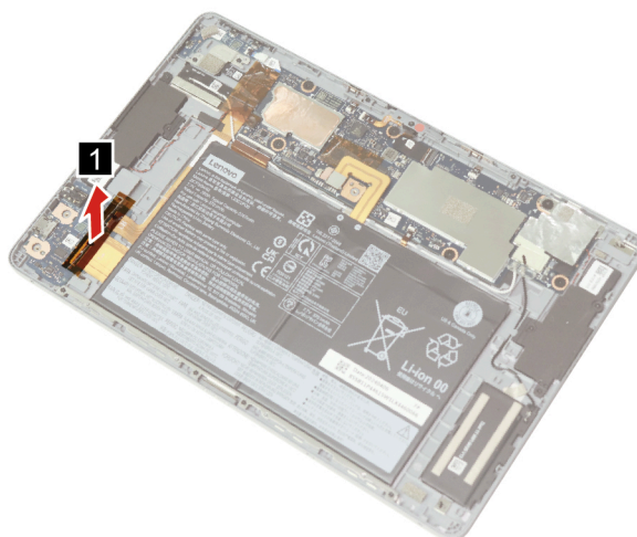
Figure 20. Peel off the mylar
