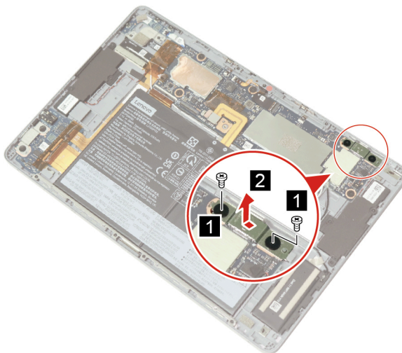
Figure 14. Remove two screws and the system board USB Type-C bracket
