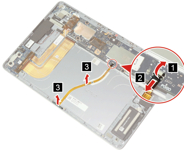
Figure 12. Disconnect and remove the pogo pin cable
