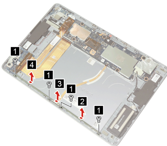
Figure 11. Remove four screws and remove the pogo pin bracket
