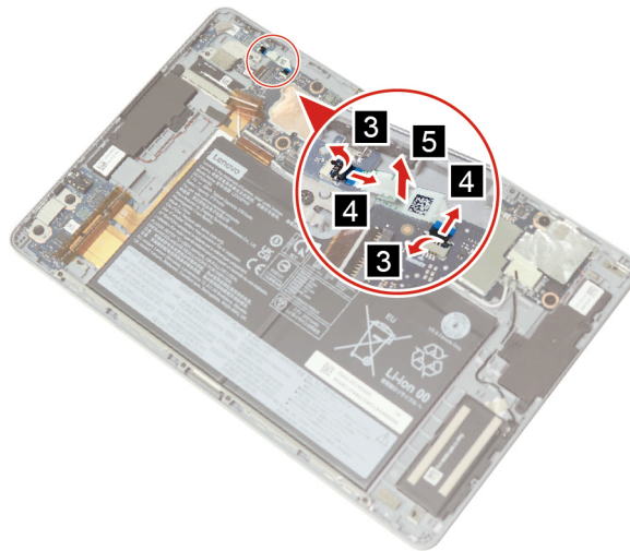
Figure 26. Disconnect and remove the power and volume board cable
