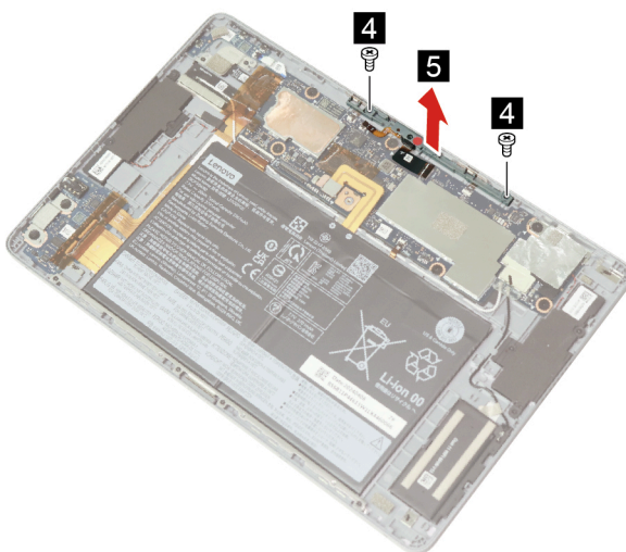
Figure 29. Remove two screws and the camera cover bracket
