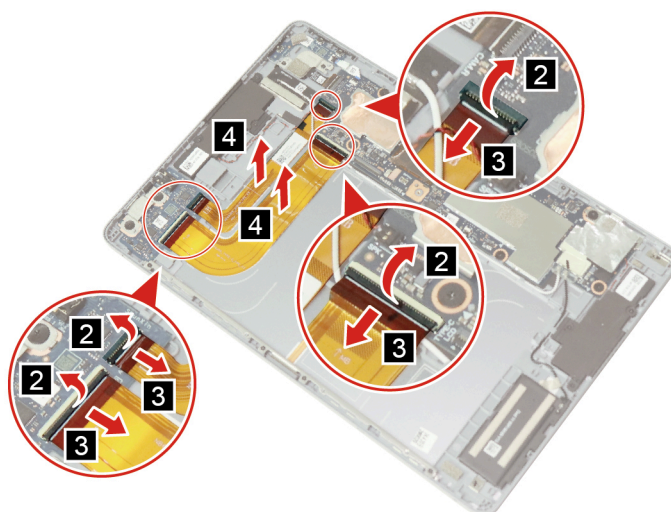
Figure 24. Disconnect and remove the USB Type-C cable and audio cable
