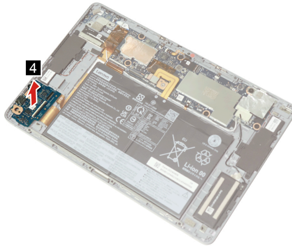
Figure 22. Remove the I/O board
