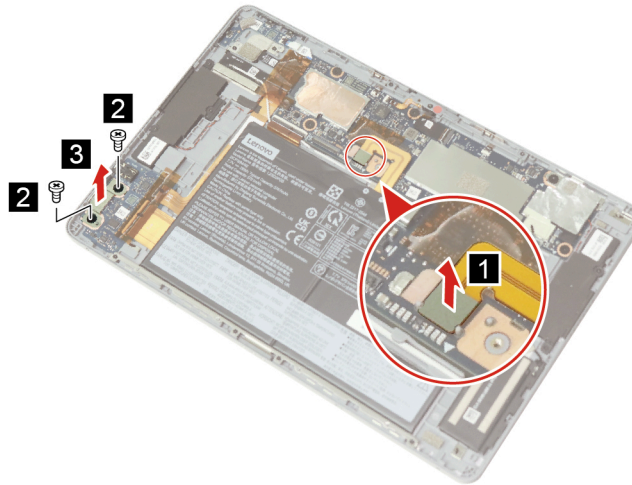
Figure 19. Disconnect the battery cable, remove two screws and the I/O board bracket
