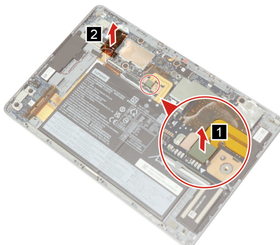
Figure 25. Disconnect the battery cable and peel off the mylar
