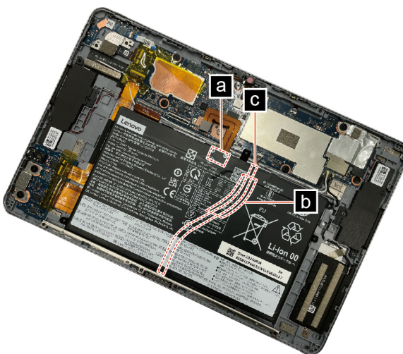
Figure 10. Install the removable tapes without covering specified areas and cable
