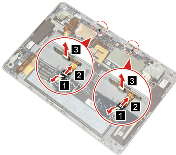
Figure 32. Disconnect and remove the microphone cables
