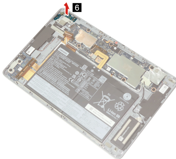
Figure 27. Remove the power and volume board
