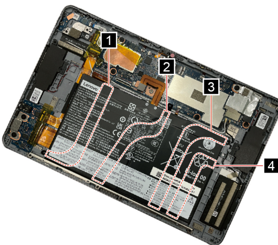
Figure 9. Install the removable tapes within specified areas
