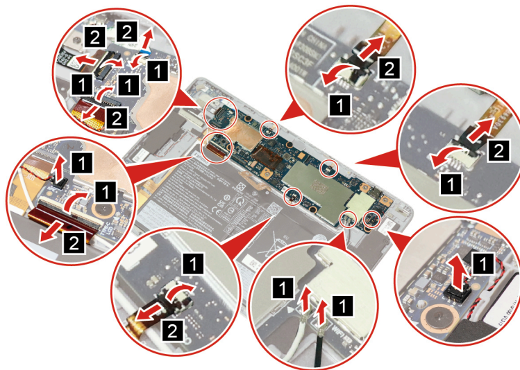
Figure 35. Disconnect cables
