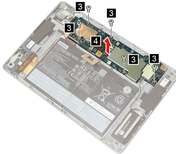
Figure 36. Remove five screws and the system board
