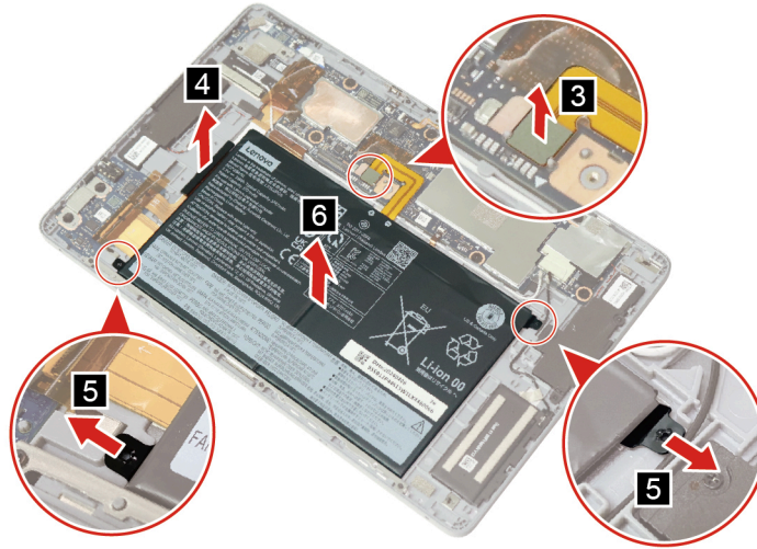
Figure 7. Disconnect the battery cable and remove the battery pack rubber, tapes, and battery pack
