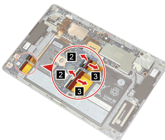
Figure 21. Disconnect the USB Type-C cable and the audio cable
