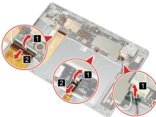
Figure 17. Disconnect the USB Type-C cable and pogo pin cable and remove the antenna cable mylar
