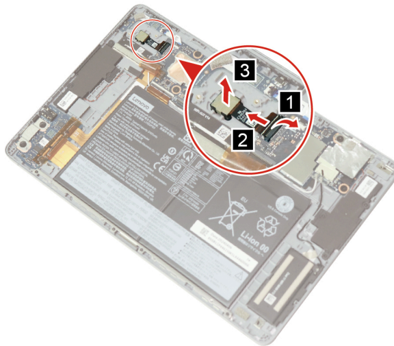
Figure 34. Disconnect and remove the rear-facing camera
