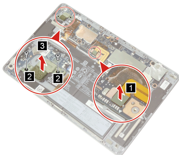
Figure 33. Disconnect the battery cable, remove two screws, and the rear-facing camera bracket
