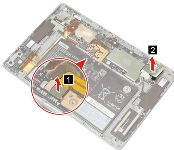
Figure 13. Disconnect the battery cable and remove the system board USB Type-C mylar
