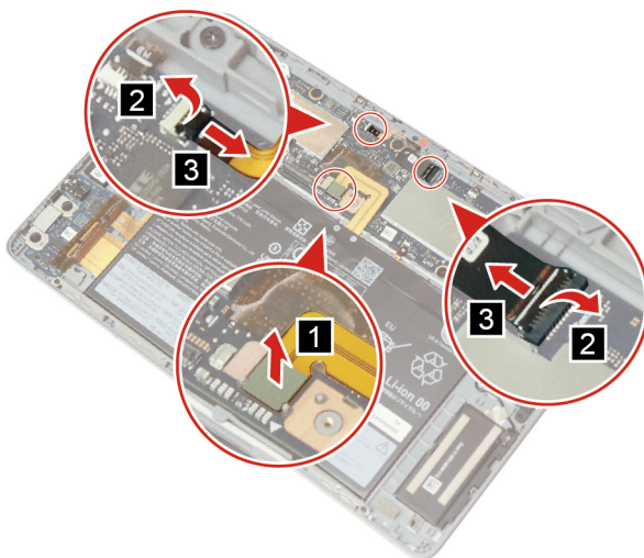
Figure 28. Disconnect the battery cable, camera, and camera LED cable
