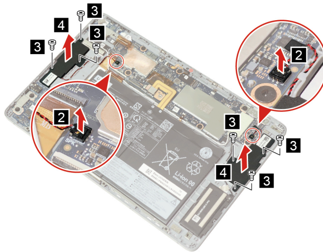
Figure 16. Disconnect and remove the speakers
