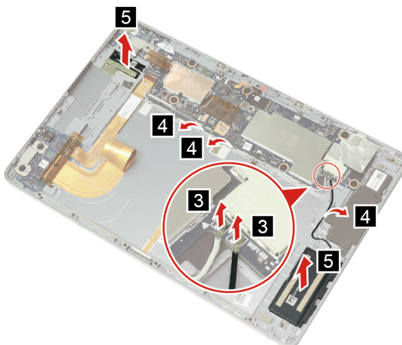
Figure 18. Remove the antennas and the antenna module
