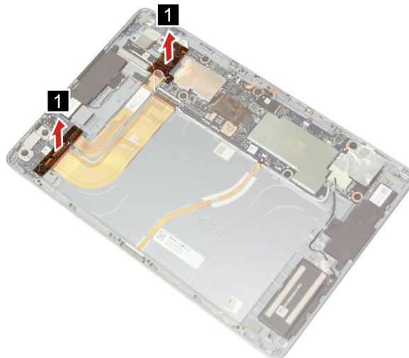
Figure 23. Peel off the mylar
