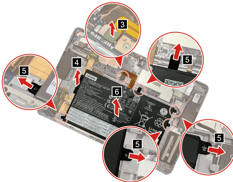
Figure 8. Disconnect the battery cable and remove the battery pack rubber, tapes, and battery pack
