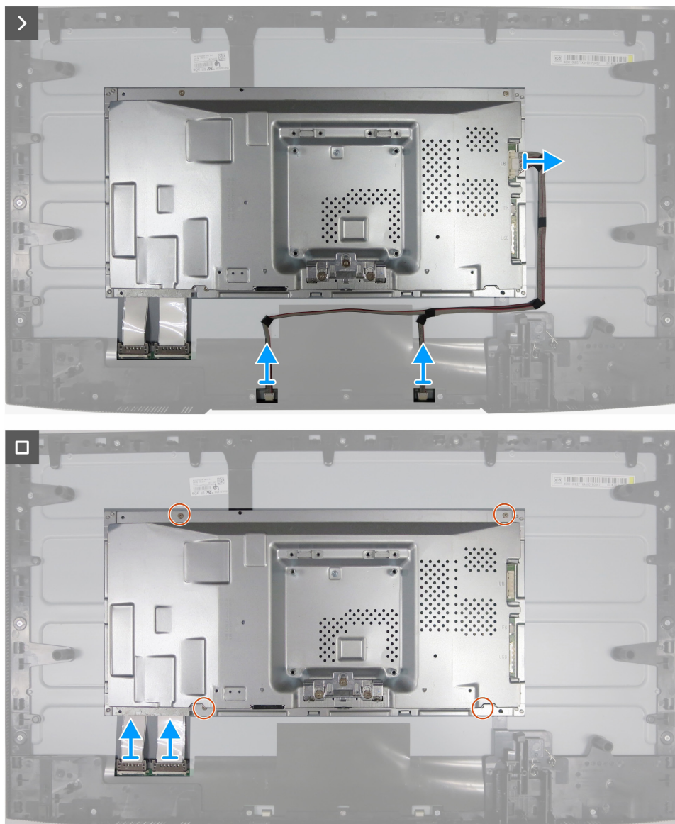
Figure 6. Removing the main chassis
