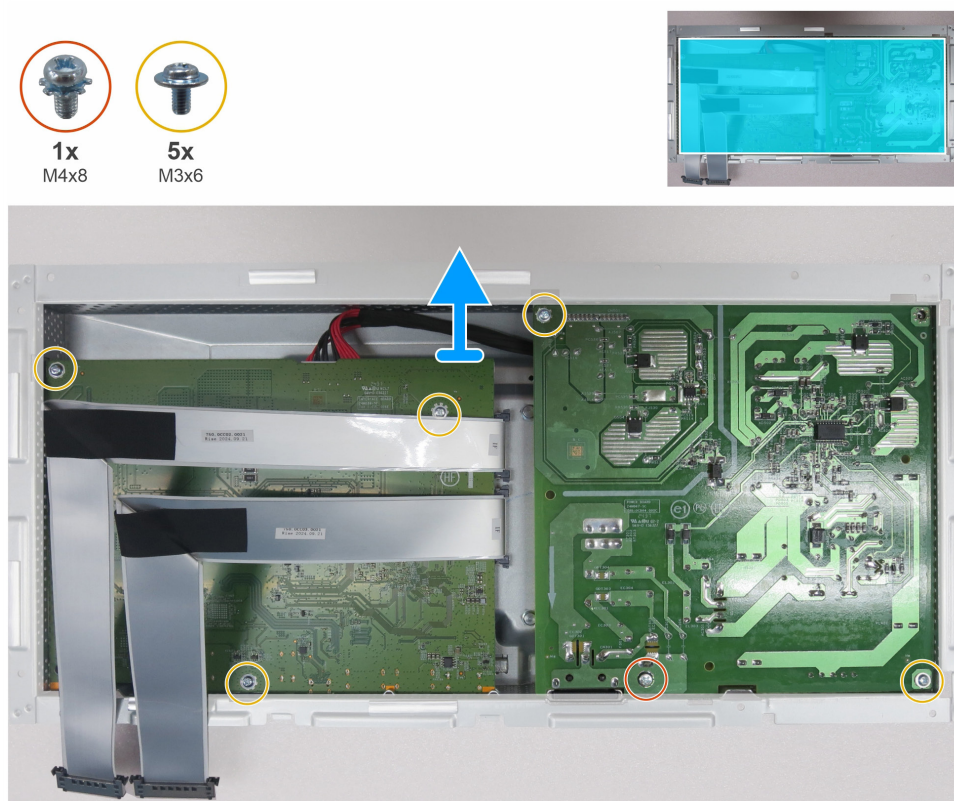
Figure 9. Removing the main board and the power board
