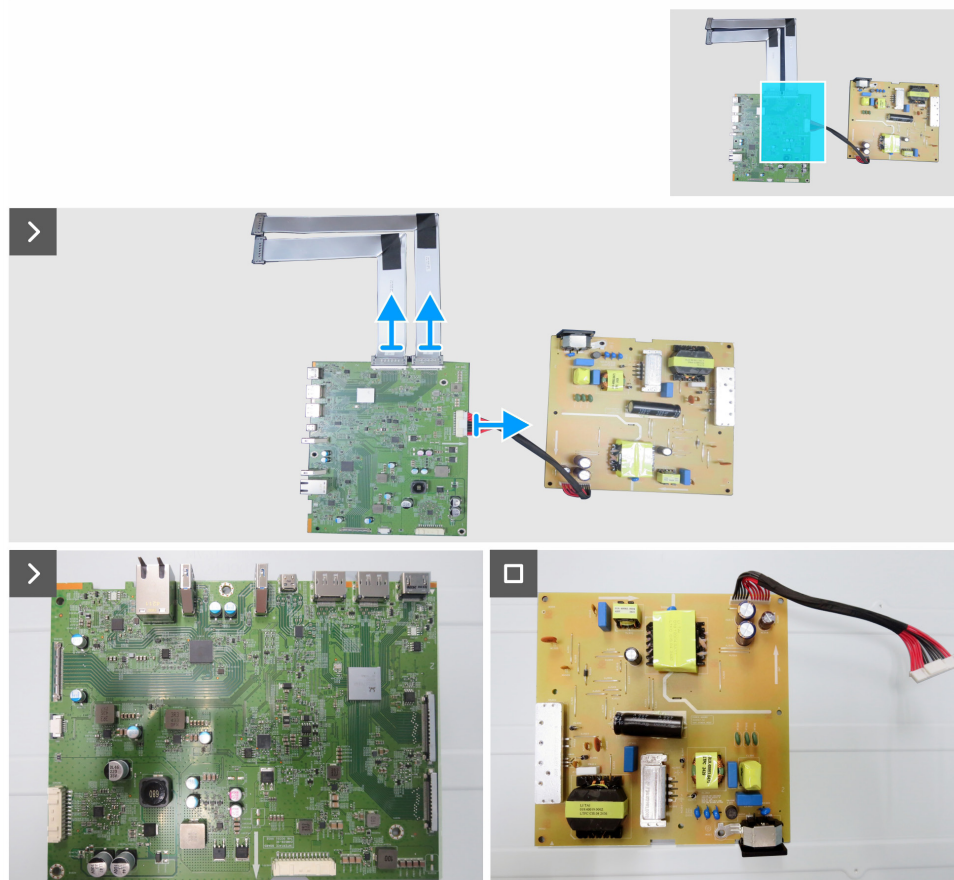
Figure 10. Disconnecting the cables from the main board
