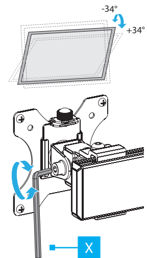
Tilt Adjustment
