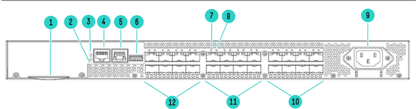
HPE Storage Fibre Channel Switch B-series SN3700B
