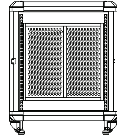
Front view (Without front door)
