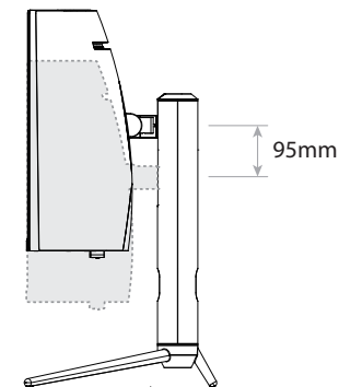
Height adjustment range 95±5mm
