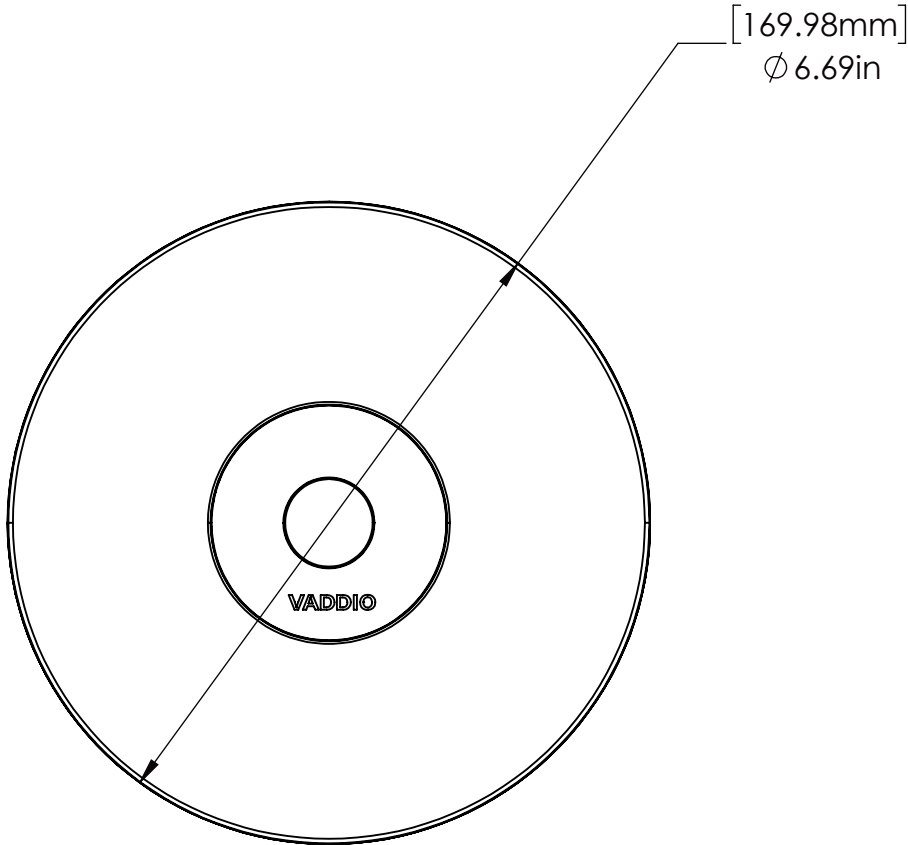
TOP VIEW
