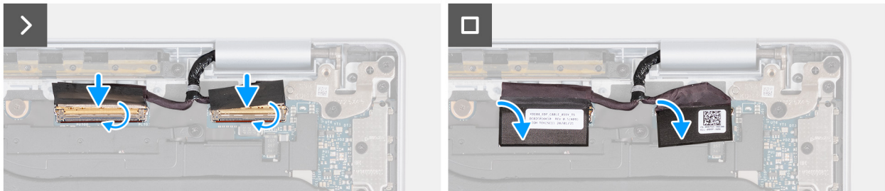
Figure 76. Installing the display assembly (for computers shipped with WLAN-only support)
