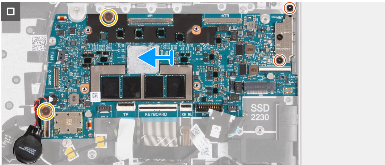
Figure 96. Removing the system board
