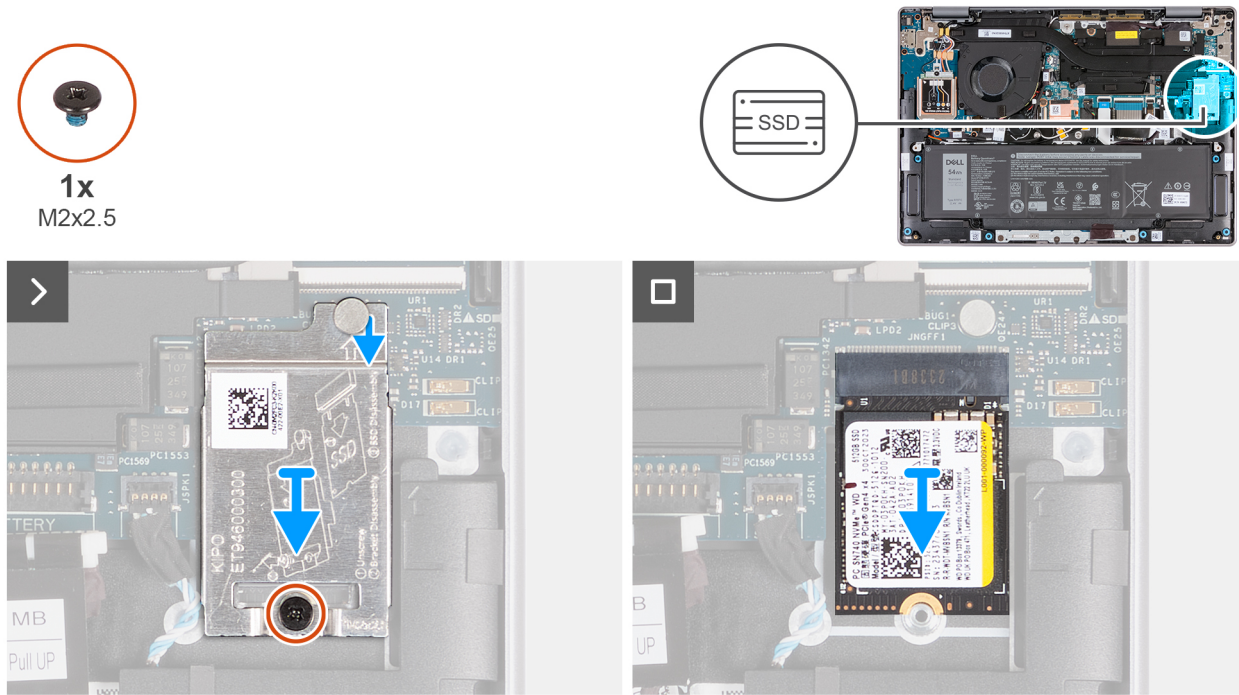
Figure 22. Removing the SSD
