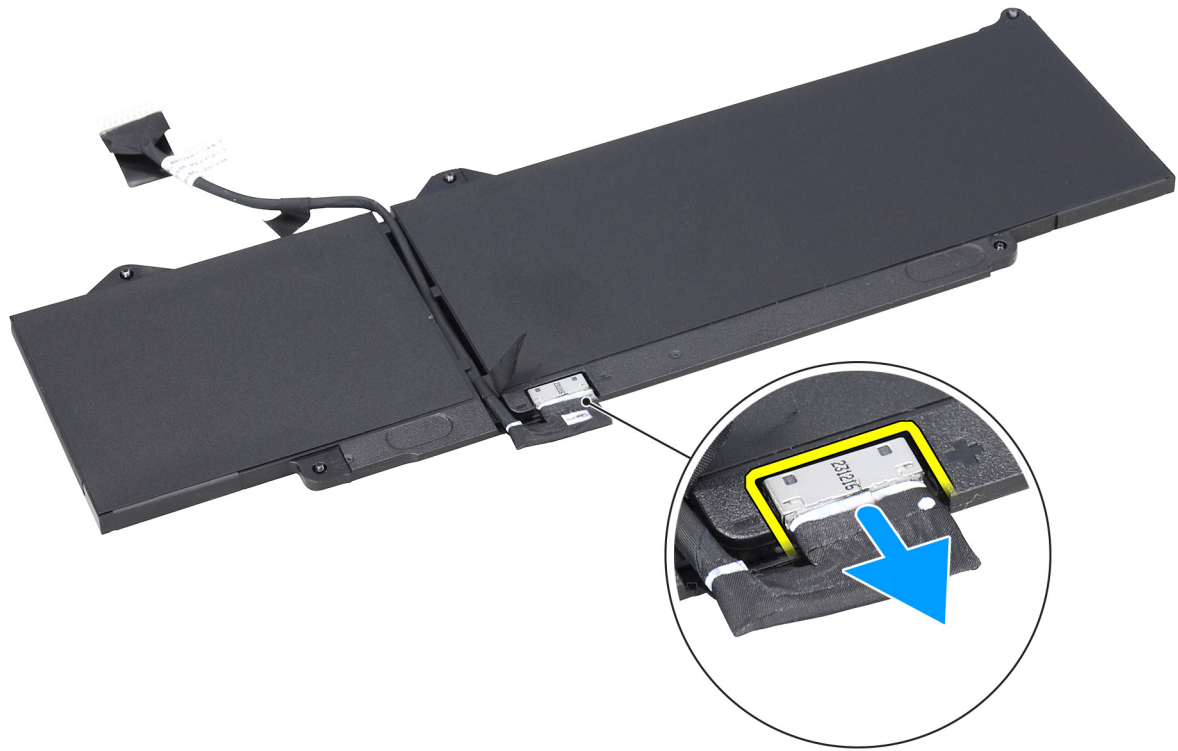
Figure 43. Disconnecting the battery cable
