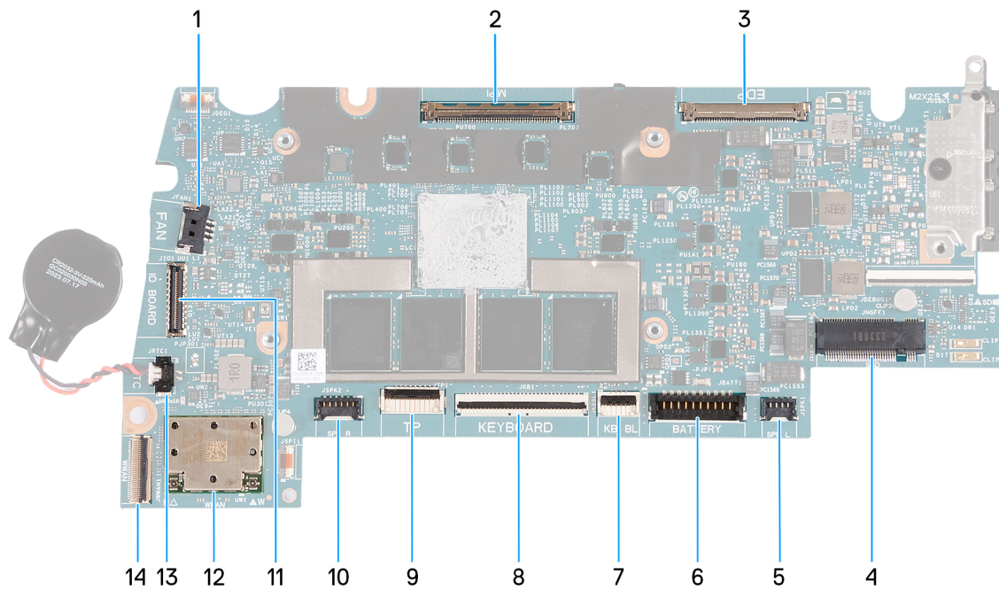
Figure 94. System-board connectors
