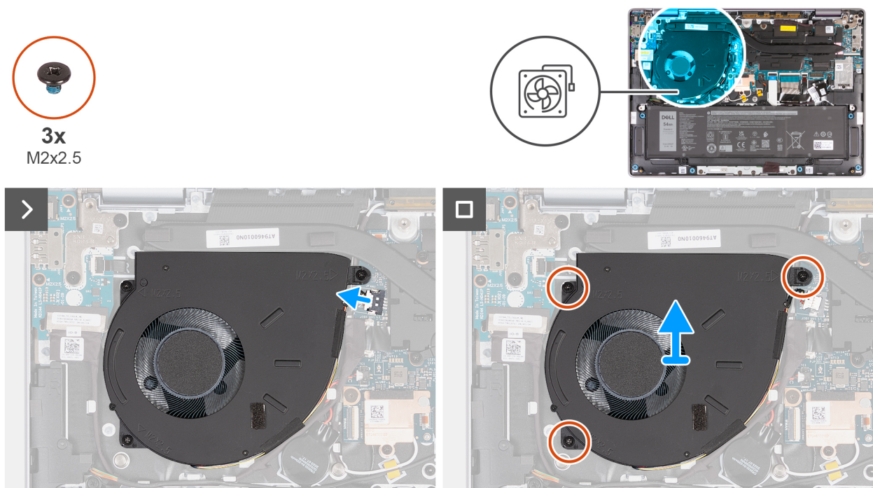
Figure 36. Removing the fan (for computers shipped with WLAN-only support)
