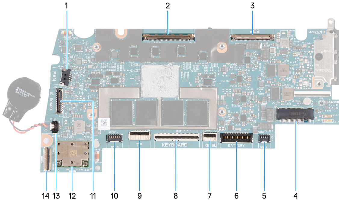
Figure 98. System-board connectors
