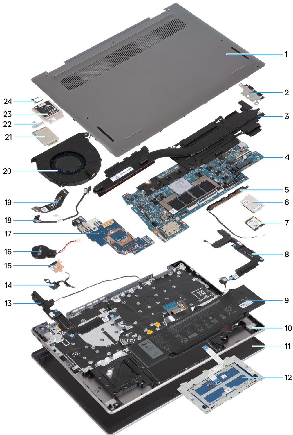
Figure 11. Major components of Latitude 7455 (computers shipped with WWAN support)
