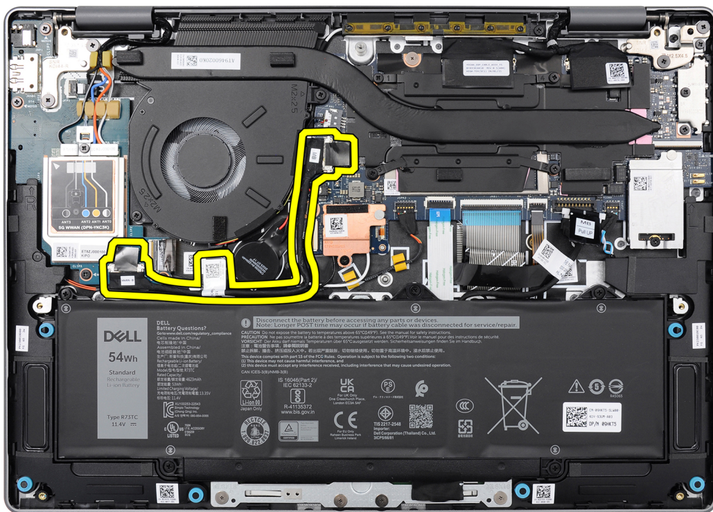
Figure 55. Location of the I/O-board cable
