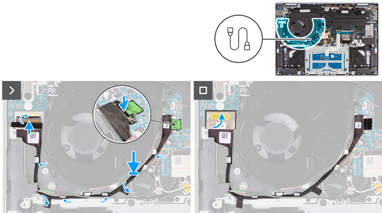
Figure 52. Installing the I/O-board cable (for computers shipped with WLAN-only support)
