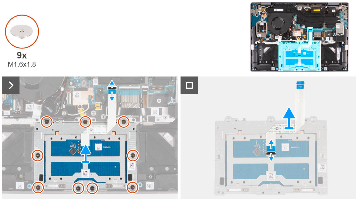
Figure 87. Removing the touchpad assembly
