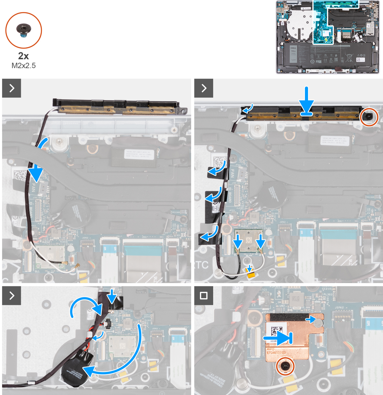
Figure 62. Installing the WLAN-antenna module (for computers shipped with WLAN-only support)
