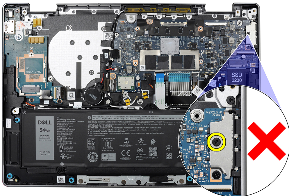
Figure 97. USB Type-C bracket
