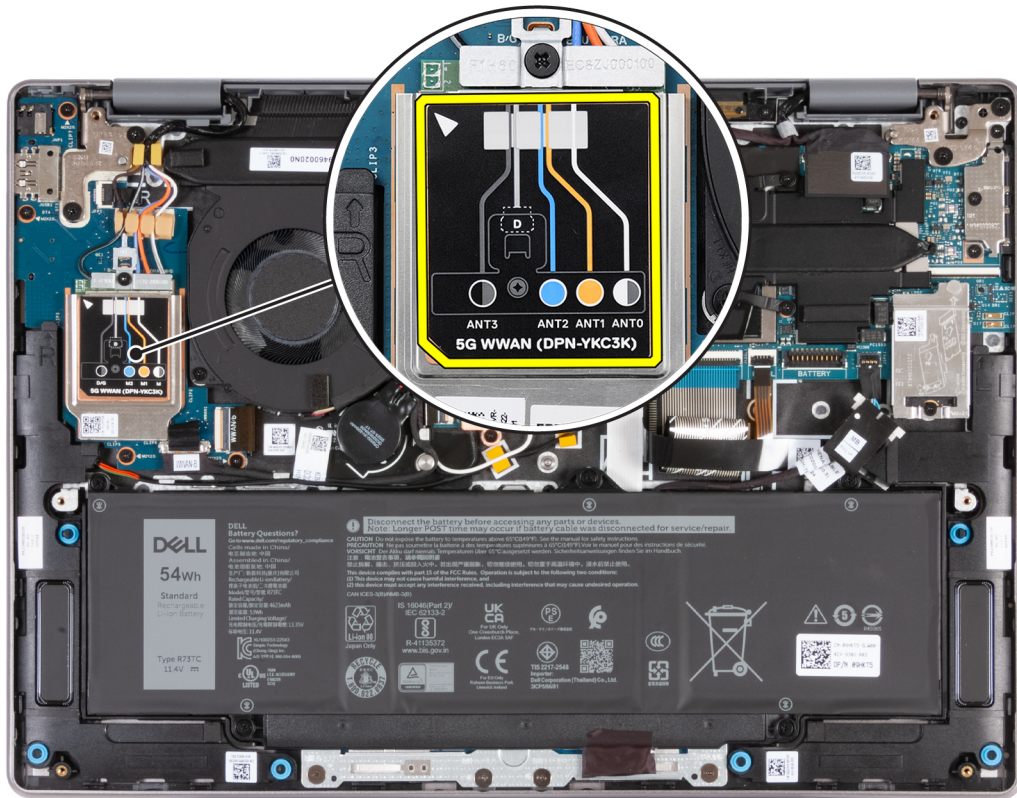
Figure 30. Antenna cable connections
