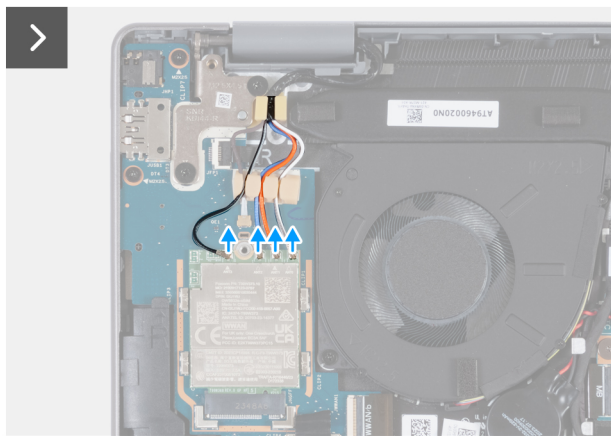
Figure 27. Removing the 5G WWAN card
