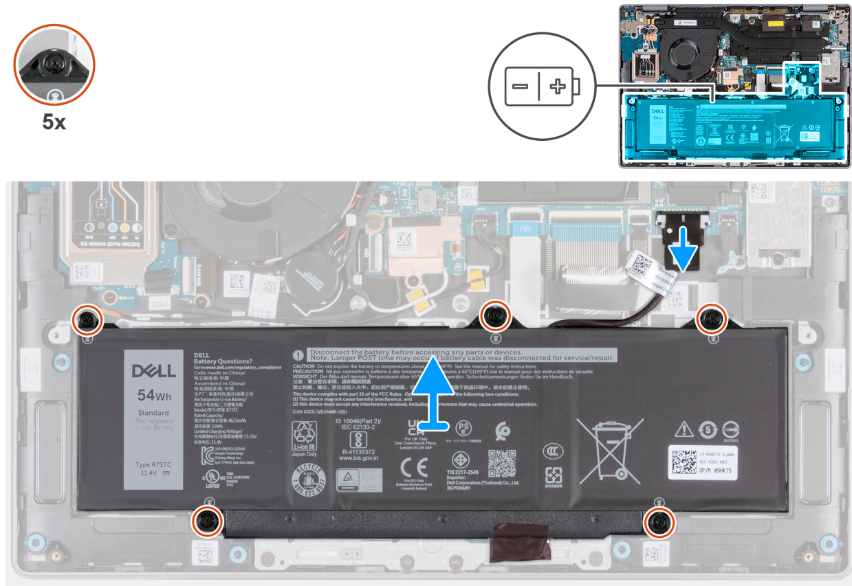
Figure 40. Removing the battery
