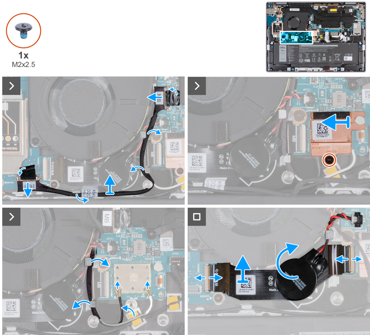
Figure 57. Removing the I/O-board FPC cable
