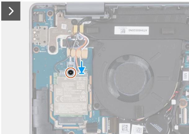
Figure 29. Installing the 5G WWAN card
