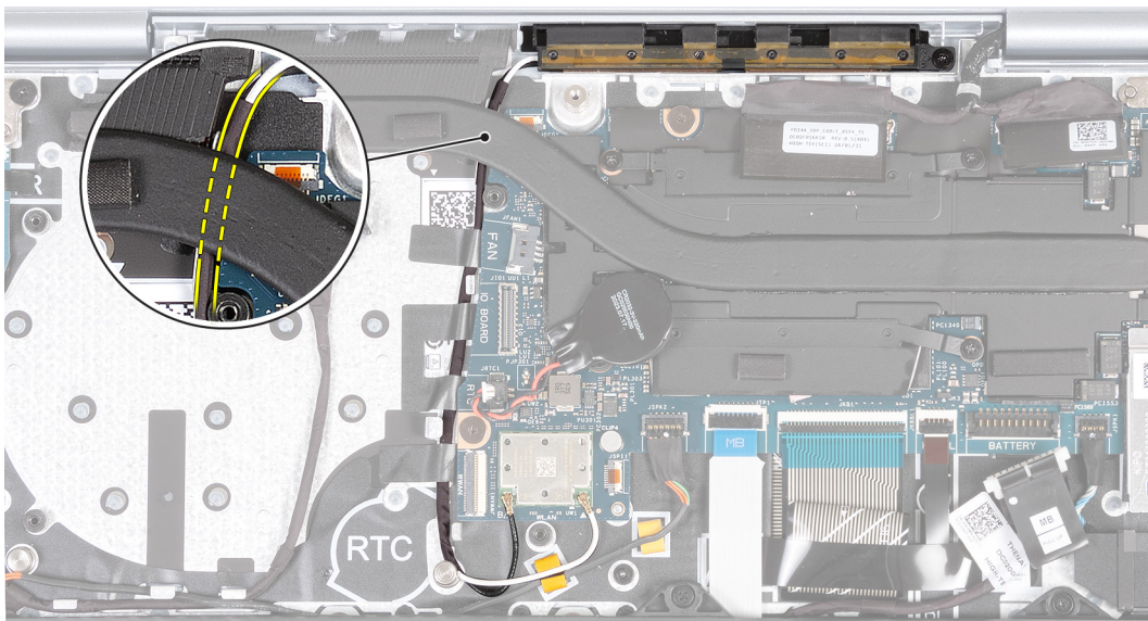
Figure 61. Removing WLAN-antenna cables
