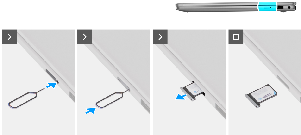
Figure 14. Removing the SIM-card tray
