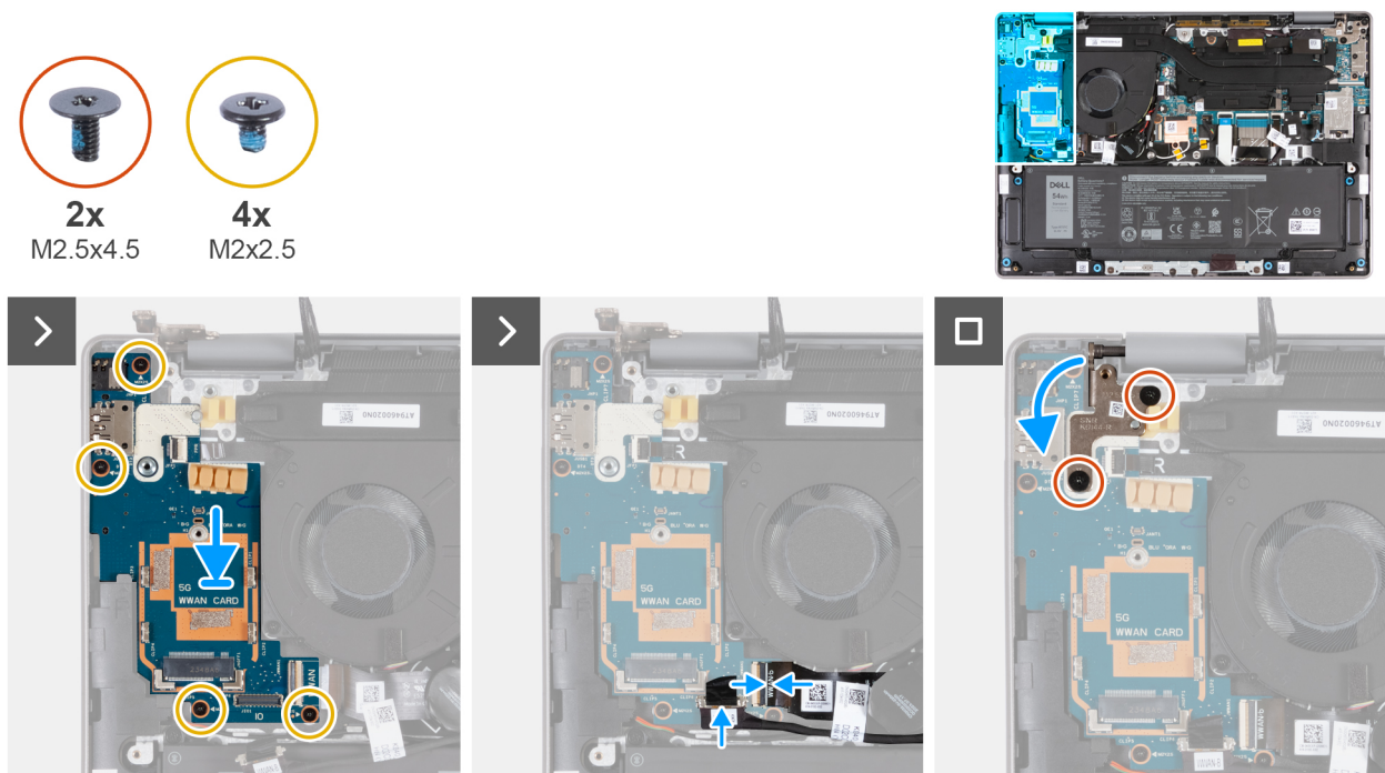
Figure 86. Installing the I/O board Removing the I/O board (for computers shipped with WWAN support)
