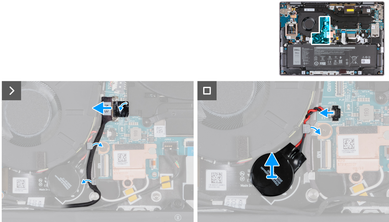
Figure 47. Removing the coin-cell battery
