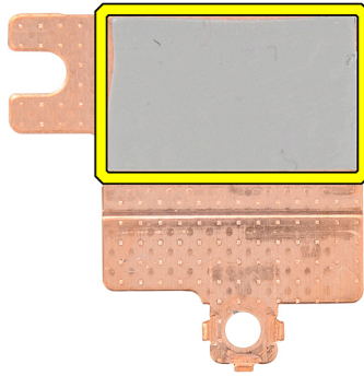
Figure 64. Thermal pad below the WLAN-thermal shield
