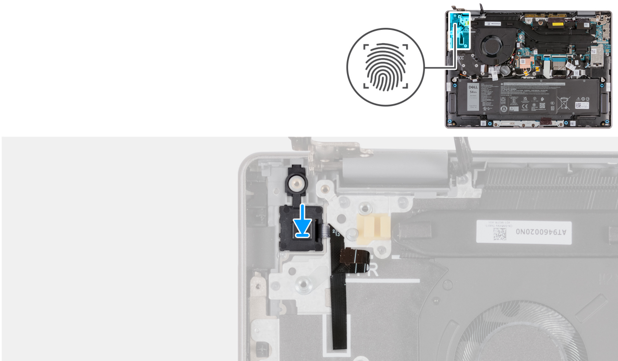
Figure 92. Installing the power button with fingerprint reader
