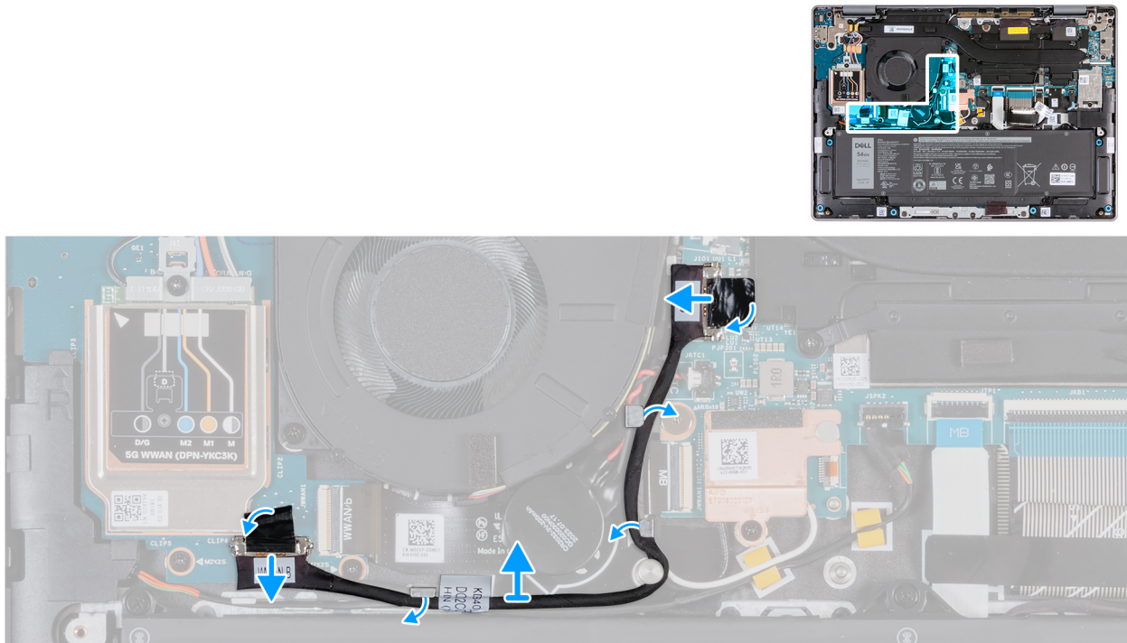
Figure 54. Removing the I/O board cable (for computers shipped with WWAN support)
