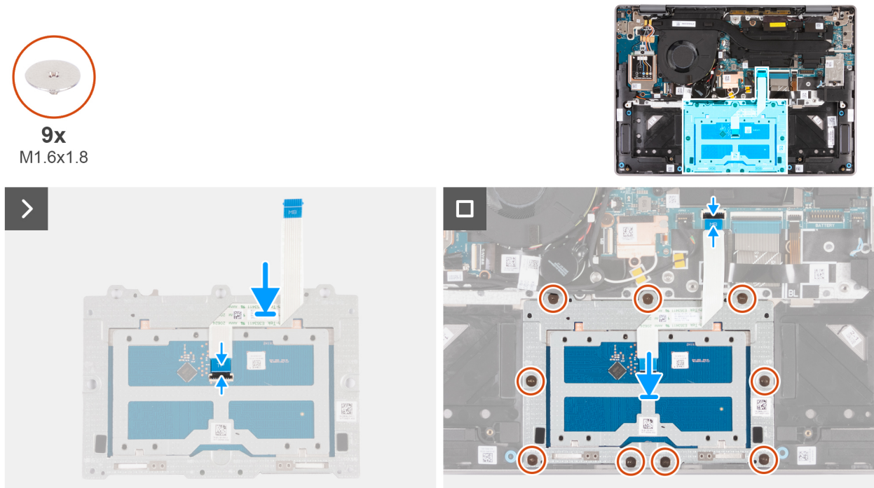
Figure 88. Installing the touchpad assembly
