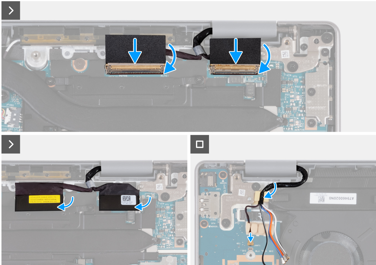
Figure 82. Installing the display assembly (for computers shipped with WWAN support)
