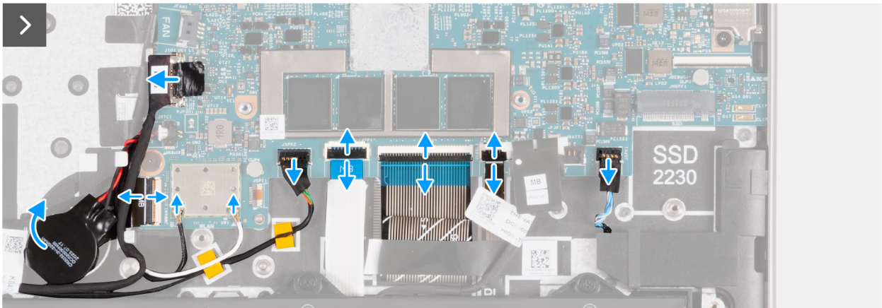
Figure 95. Removing the system board
