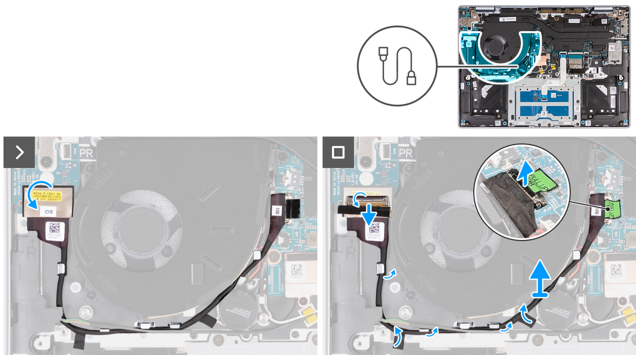
Figure 50. Removing the I/O-board cable (for computers shipped with WLAN-only support)
