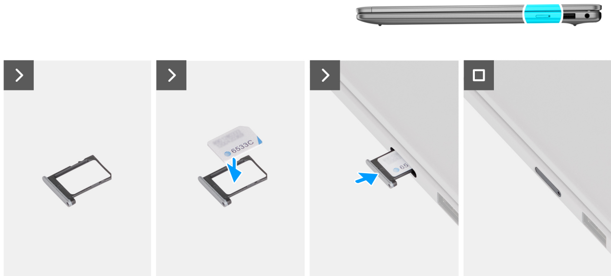
Figure 15. Installing the SIM-card tray
