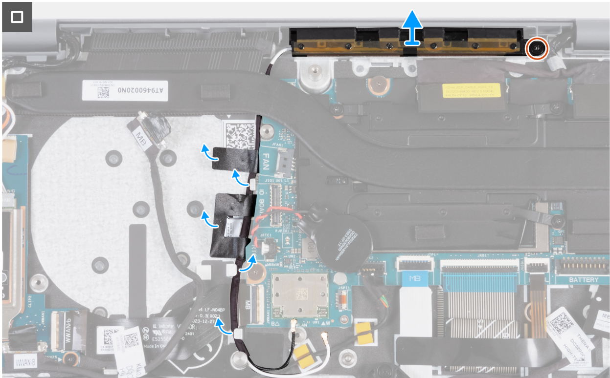
Figure 67. Removing the WLAN-antenna module
