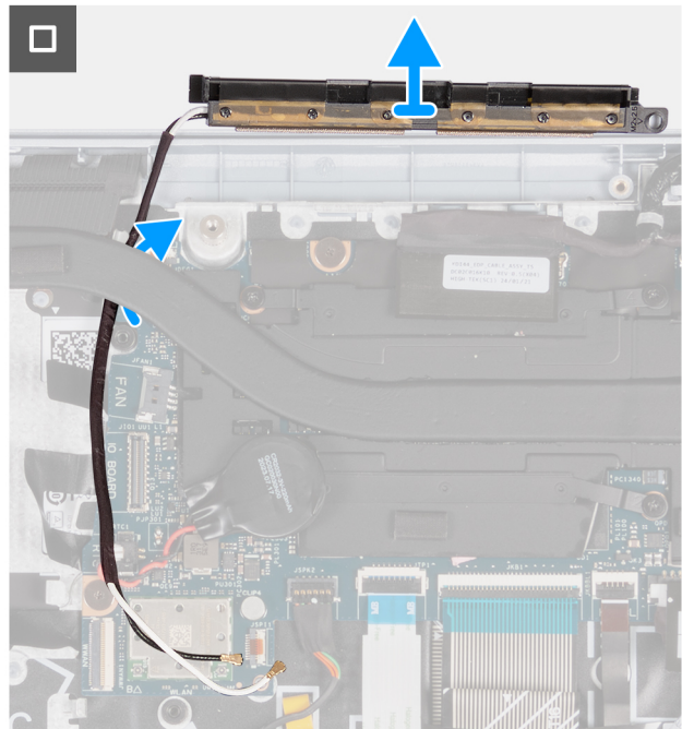
Figure 59. Removing the WLAN-antenna module (for computers shipped with WLAN-only support)
