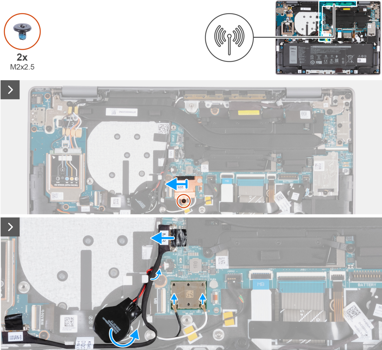
Figure 66. Removing the WLAN-antenna module
