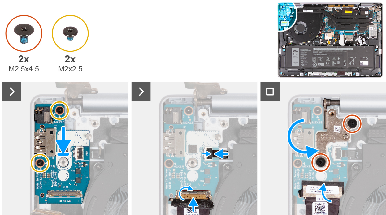
Figure 84. Installing the I/O board (for computers shipped with WLAN-only support)
