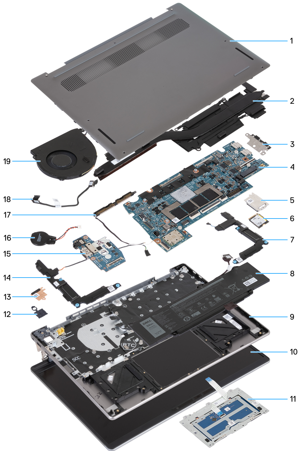
Figure 10. Major components of Latitude 7455 (computers shipped with WLAN-only support)
