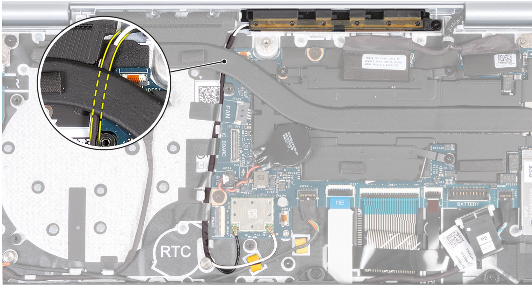
Figure 69. Removing WLAN-antenna cables
