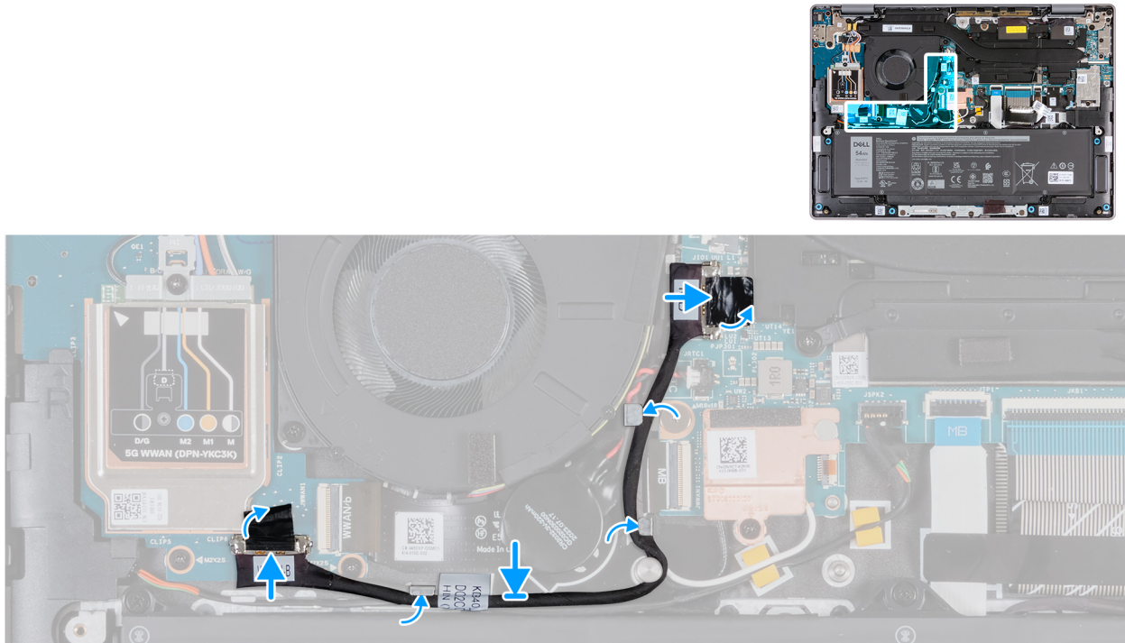
Figure 56. Installing the I/O-board cable (for computers shipped with WWAN support)
