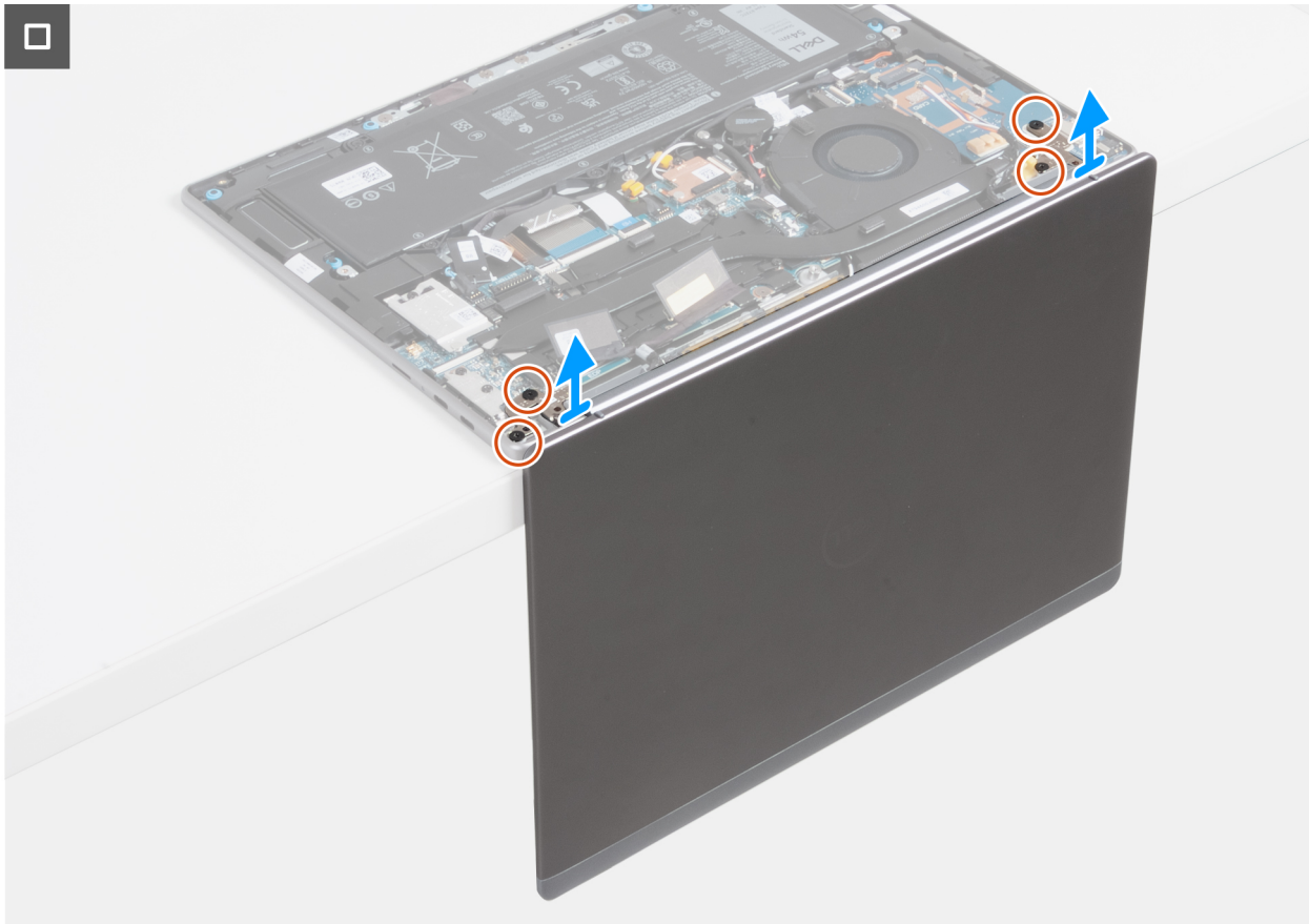
Figure 79. Removing the display assembly (for computers shipped with WWAN support)
