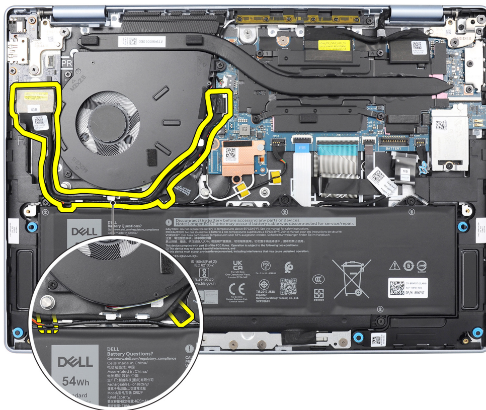
Figure 51. Location of the I/O-board cable
