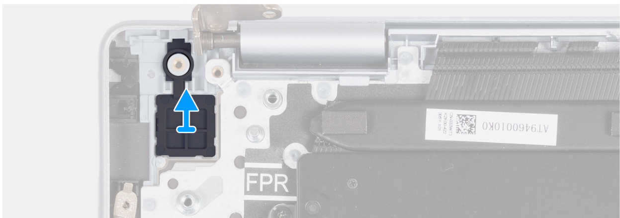
Figure 89. Removing the power button
