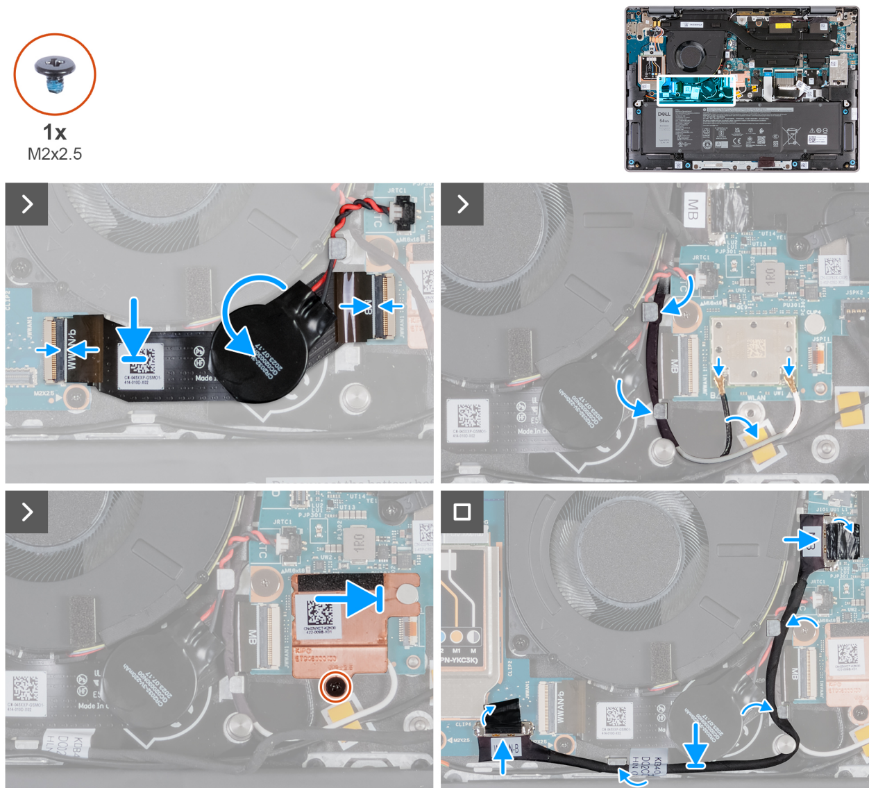
Figure 58. Installing the I/O-board FPC cable
