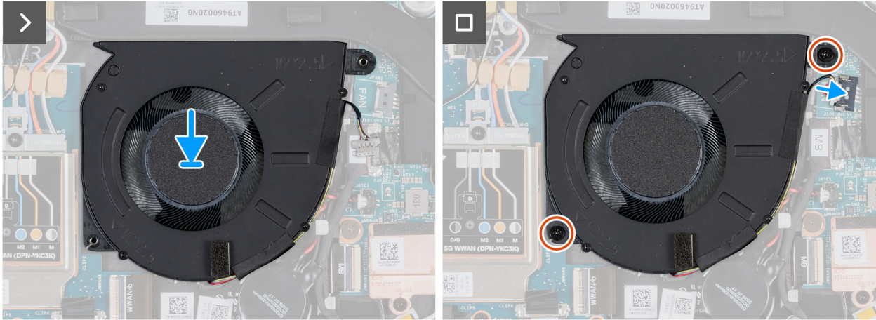
Figure 39. Installing the fan (for computers shipped with WWAN support)
