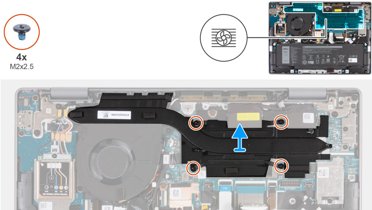
Figure 45. Removing the heat sink
