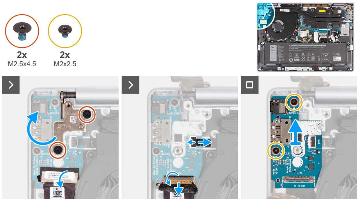
Figure 83. Removing the I/O board (for computers shipped with WLAN-only support)
