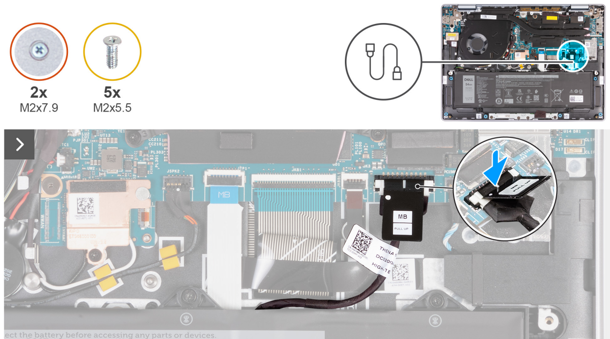
Figure 19. Connecting the battery cable
