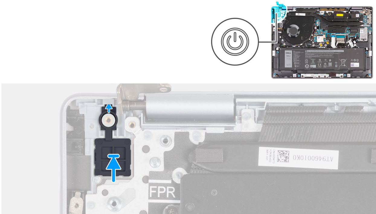
Figure 91. Installing the power button
