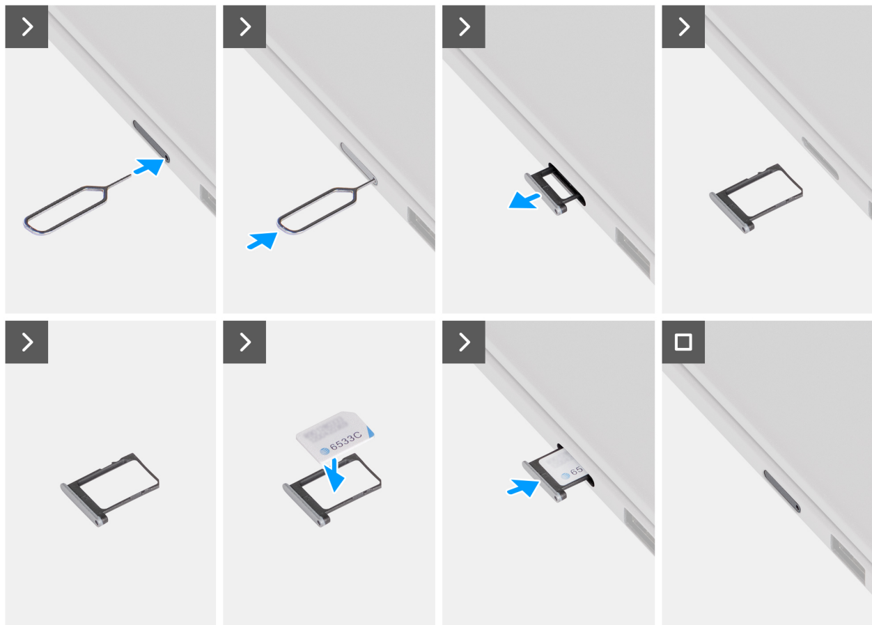
Figure 13. Installing the SIM card
