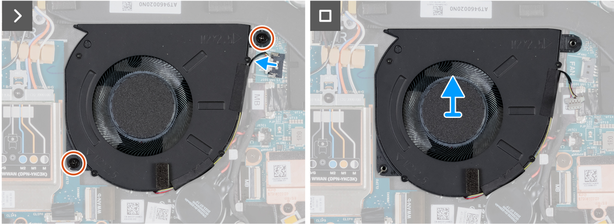
Figure 38. Removing the fan (for computers shipped with WWAN support)
