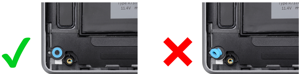
Figure 35. Installation of rubber grommets
