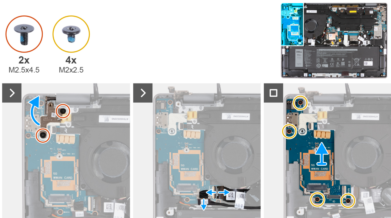
Figure 85. Removing the I/O board (for computers shipped with WWAN support)
