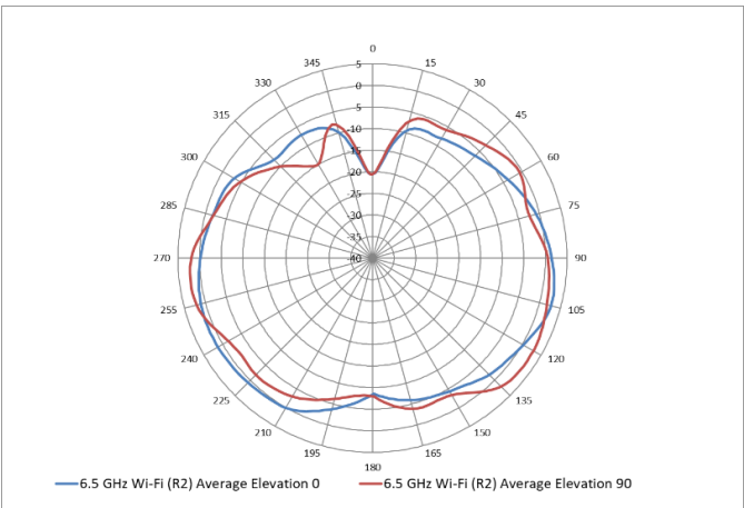
6.5 GHz Wi-Fi antennas patterns (vertical)
