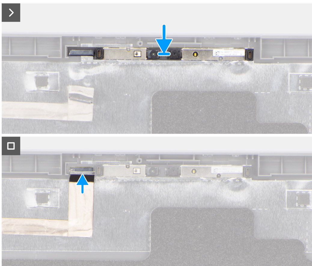
Figur 67. Installera kameran
