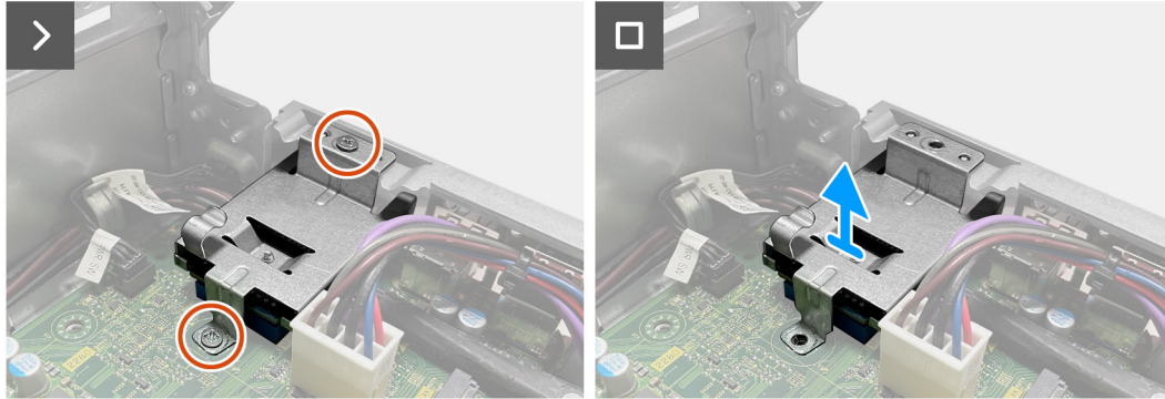
Figure 36. Removing the media-card reader
