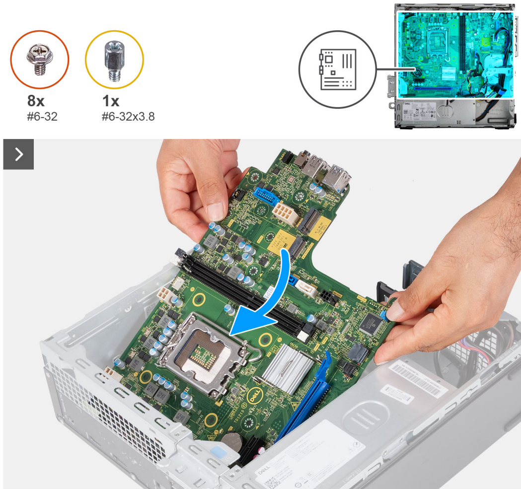
Figure 57. Placing the system board in the chassis
