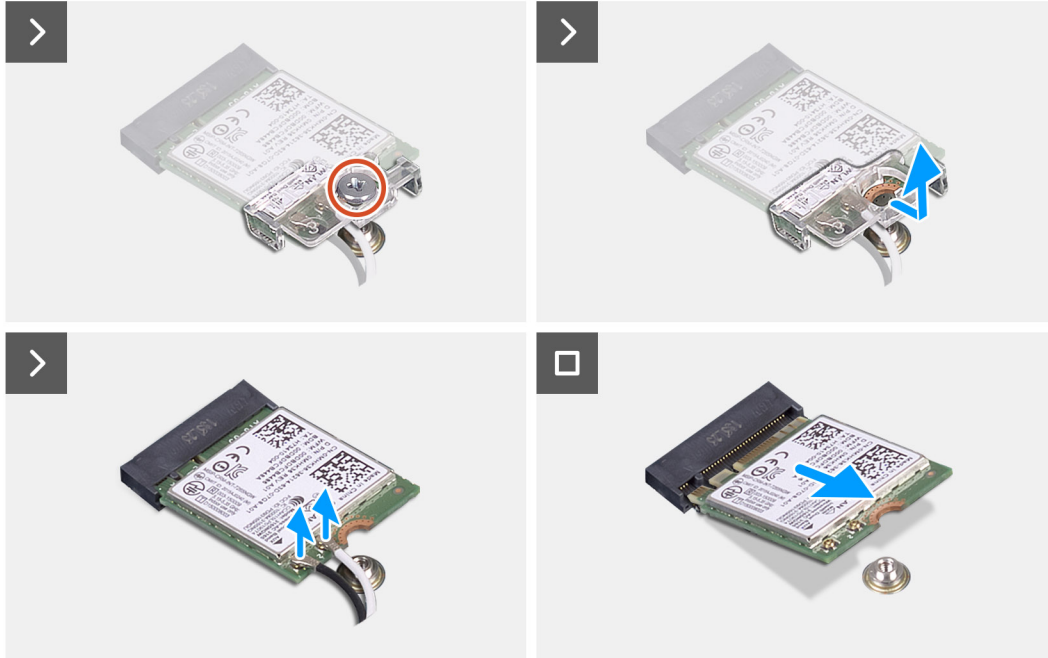
Figure 32. Removing the wireless card
