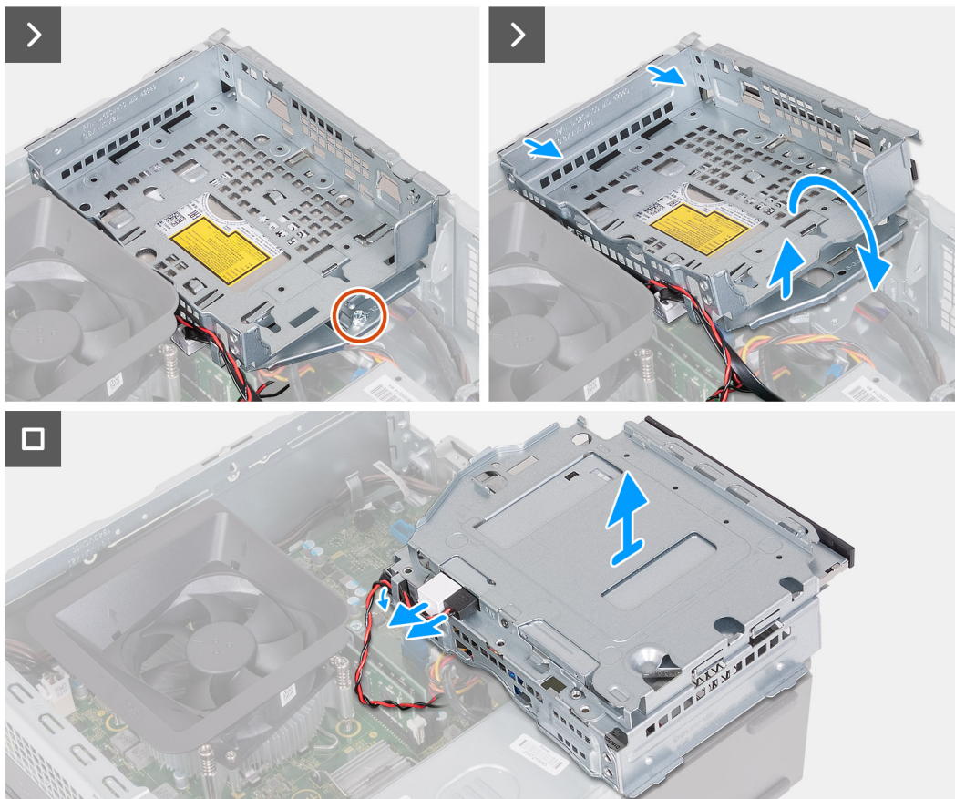
Figure 18. Removing the hard-drive and optical-drive cage
