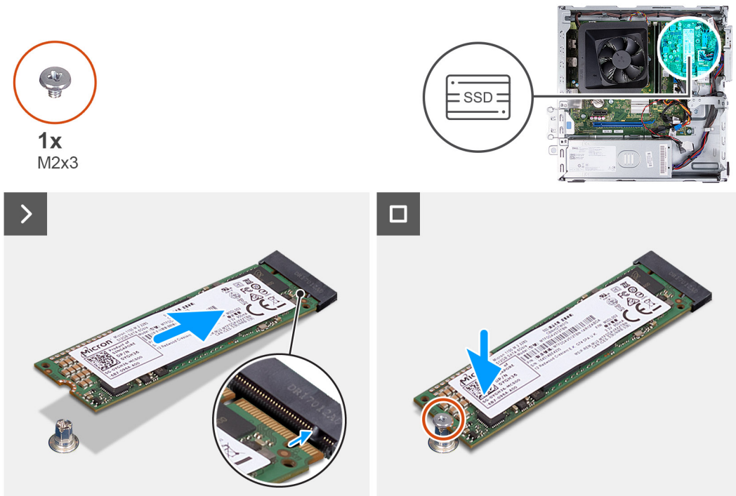
Figure 31. Installing the M.2 2280 solid-state drive
