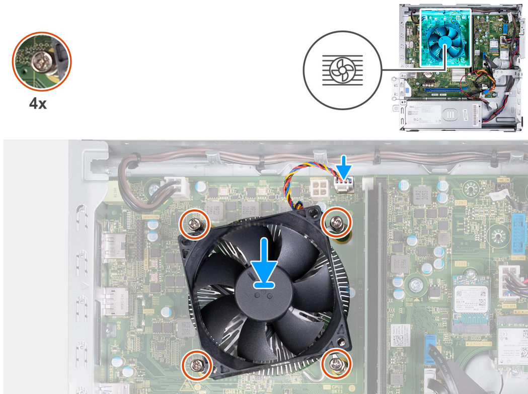
Figure 49. Installing the fan and heat-sink assembly
