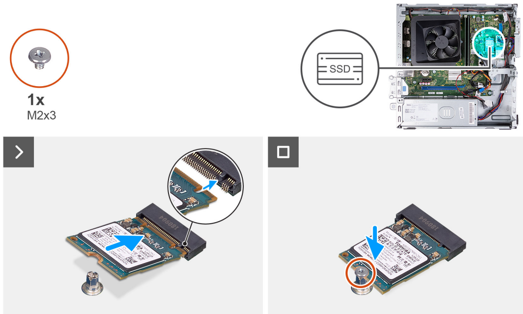
Figure 28. Installing the M.2 2230 solid-state drive
