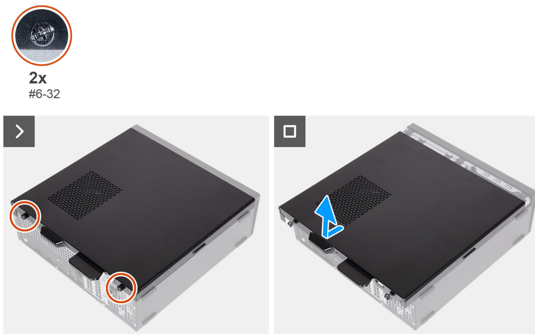
Figure 12. Removing the left-side cover
