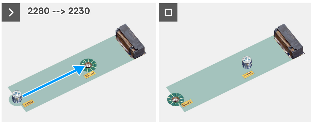
Figure 27. Fixing screw mount 2280 to 2230
