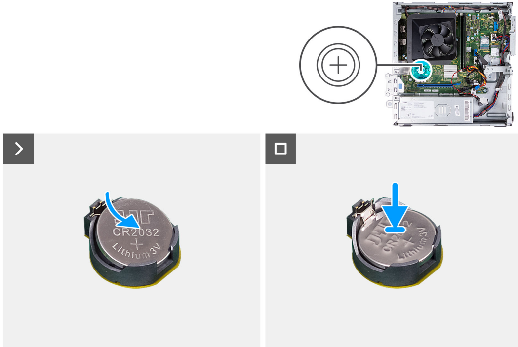
Figure 11. Installing the coin-cell battery
