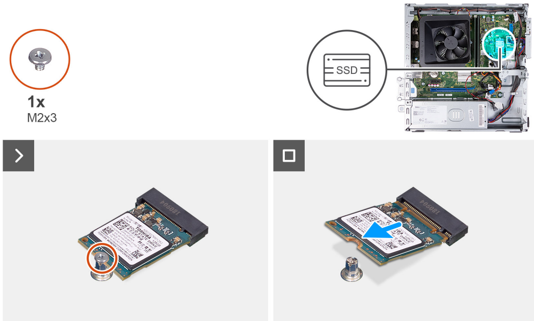
Figure 26. Removing the M.2 2230 solid-state drive
