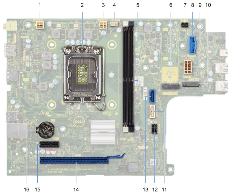
Figure 56. System-board connectors
