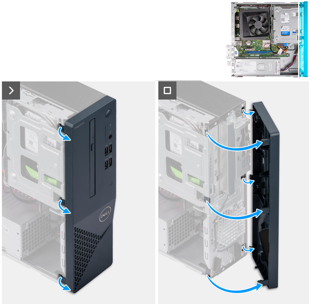
Figure 14. Removing the front cover
