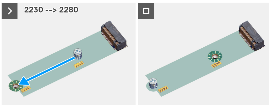
Figure 30. Fixing screw mount 2230 to 2280
