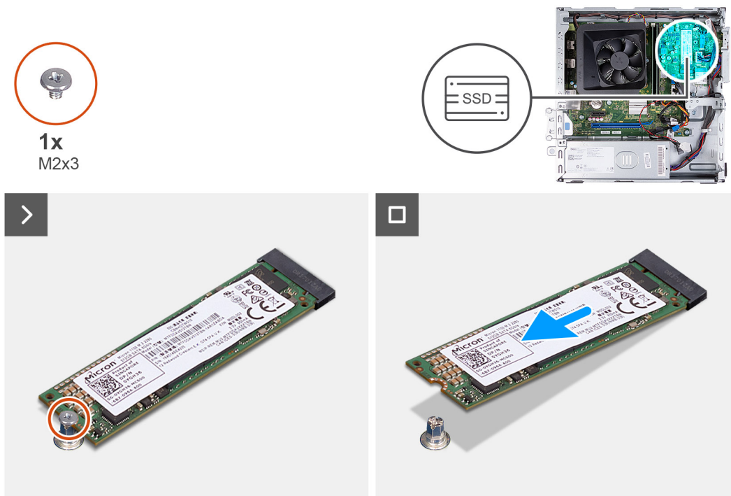
Figure 29. Removing the M.2 2280 solid-state drive
