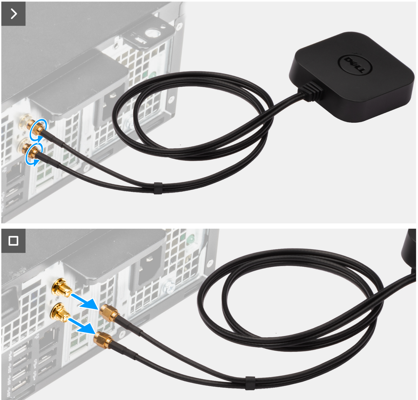
Figure 38. Removing the external antenna
