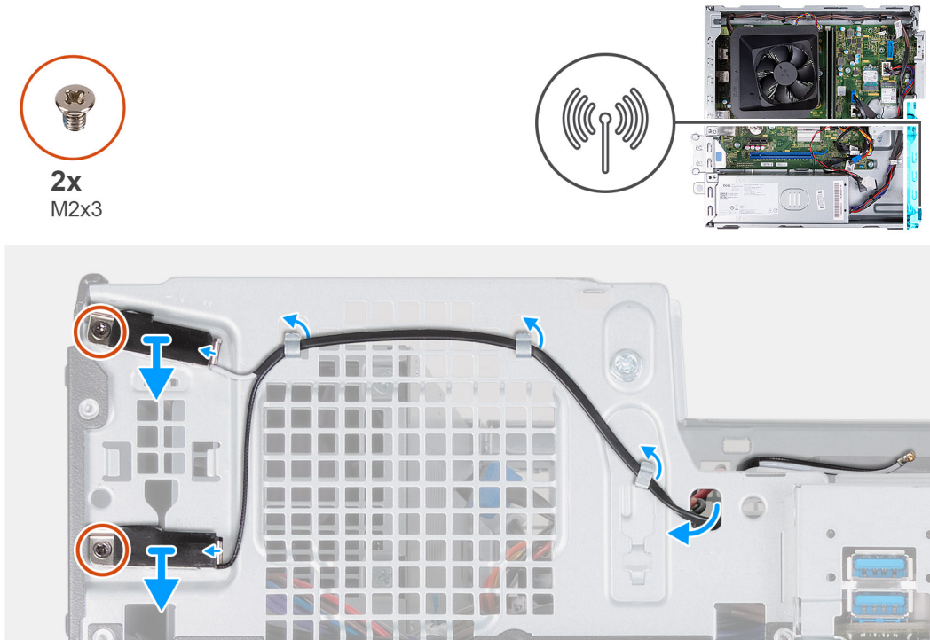
Figure 44. Removing the antenna module
