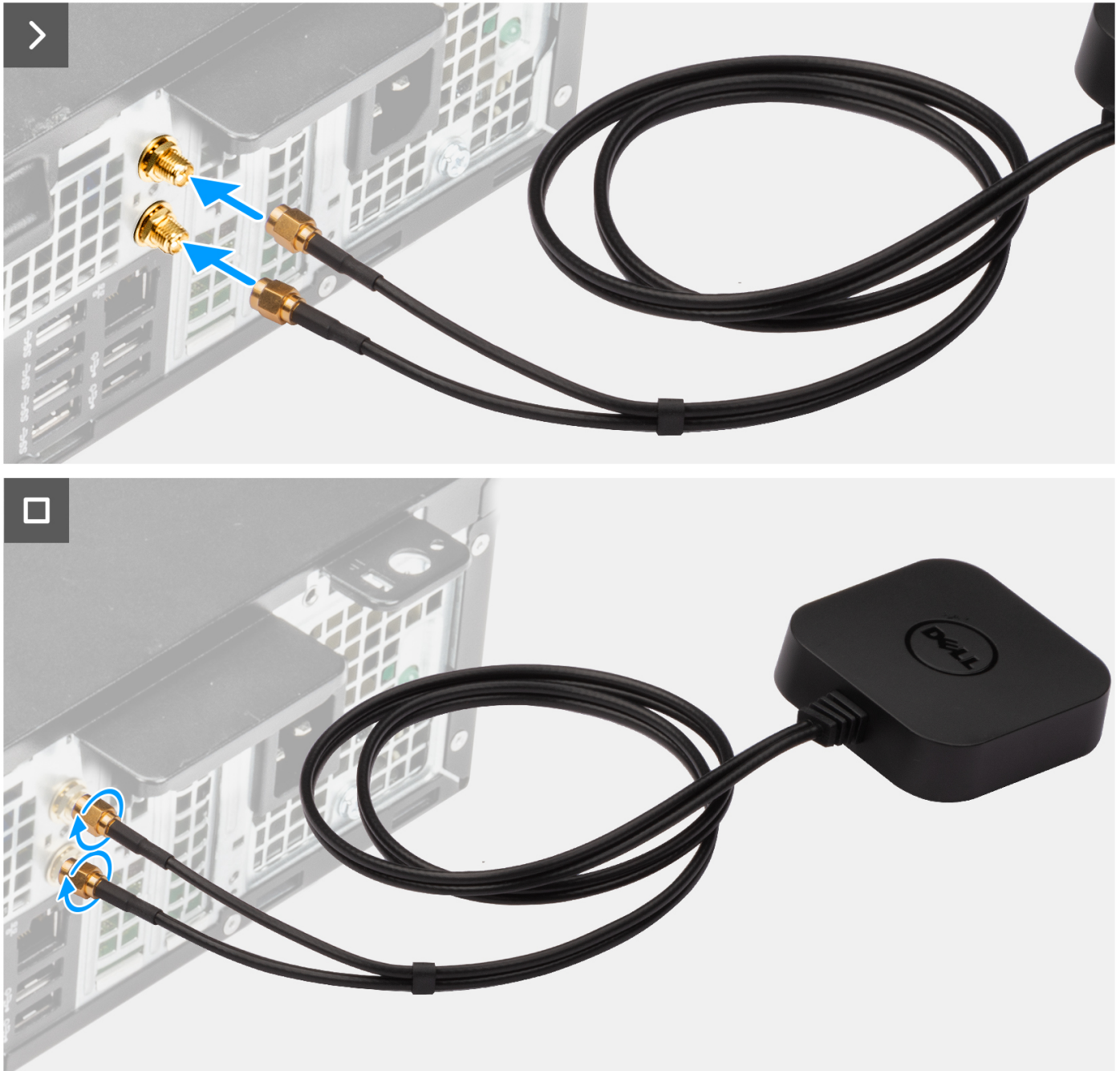
Figure 39. Installing the external antenna
