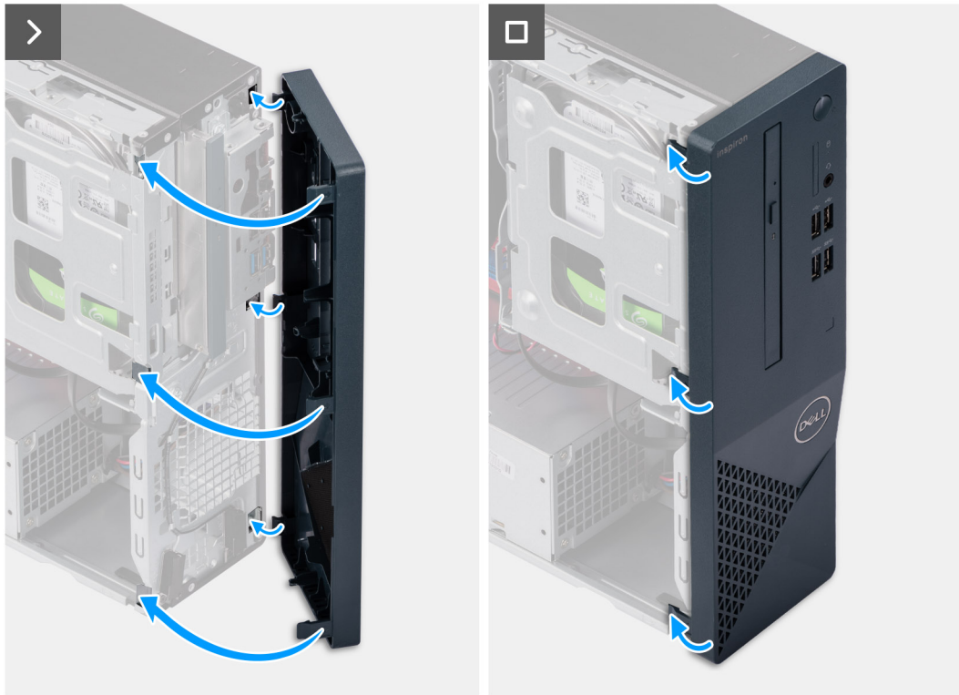
Figure 15. Installing the front cover
