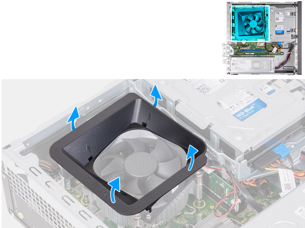
Figure 34. Removing the fan shroud
