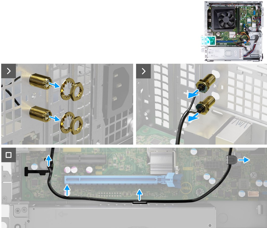
Figure 46. Removing the SMA Antenna kit
